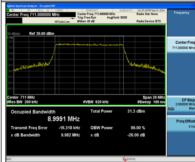
Band17-10MHz-64QAM-23800-50RB#0-PASS
