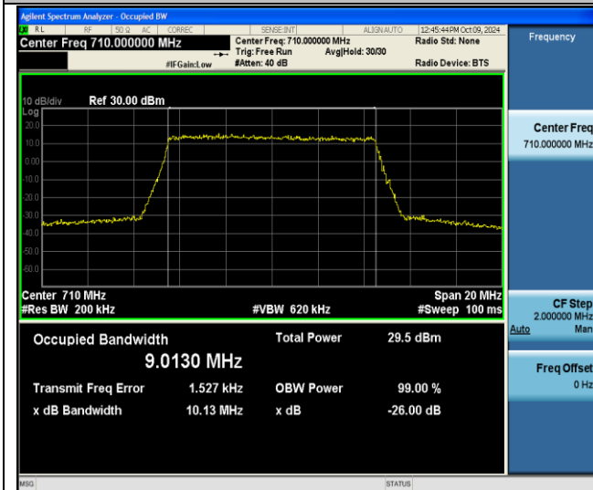
Band17-10MHz-256QAM-23790-50RB#0-PASS
