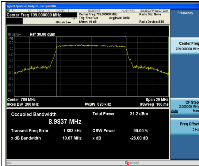
Band17-10MHz-64QAM-23780-50RB#0-PASS
