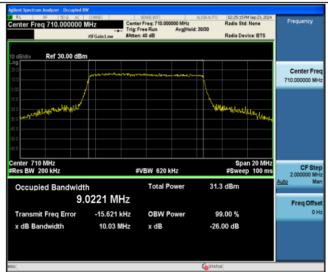
Band17-10MHz-64QAM-23790-50RB#0-PASS
