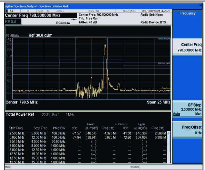
NTNV-Band14-5MHz-256QAM-23305-1RB#24--5.00--2.50-PASS
