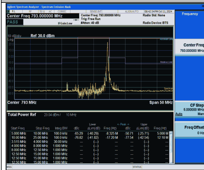
NTNV-Band14-10MHz-16QAM-23330-1RB#49--10.00--5.00-PASS
