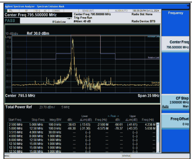
NTVN-Band14-5MHz-16QAM-23355-1RB#0--12.50--5.00-PASS
