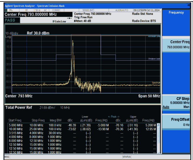
NTNV-Band14-10MHz-64QAM-23330-1RB#0--25.00--10.00-PASS
