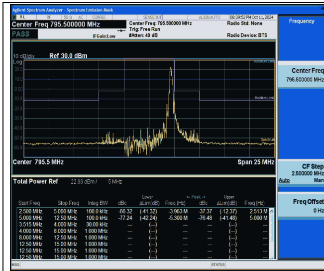
NTVN-Band14-5MHz-16QAM-23355-1RB#24-2.50-5.00-PASS
