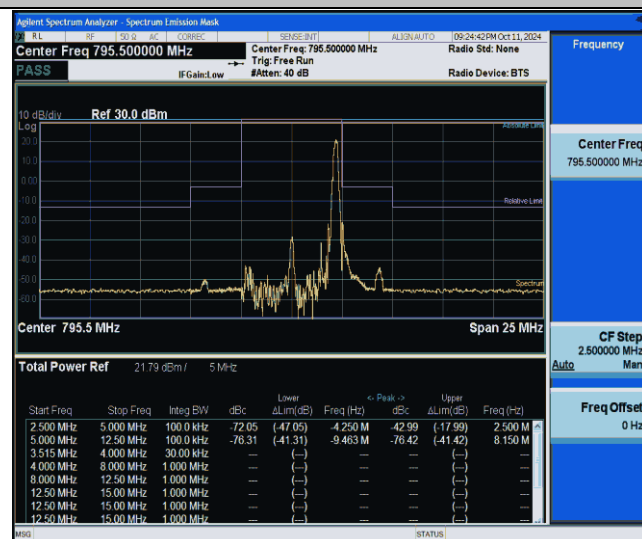
NTNV-Band14-5MHz-256QAM-23355-1RB#24-5.00-12.50-PASS
