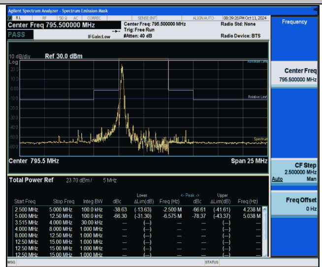
NTVN-Band14-5MHz-16QAM-23355-1RB#0-2.50-5.00-PASS
