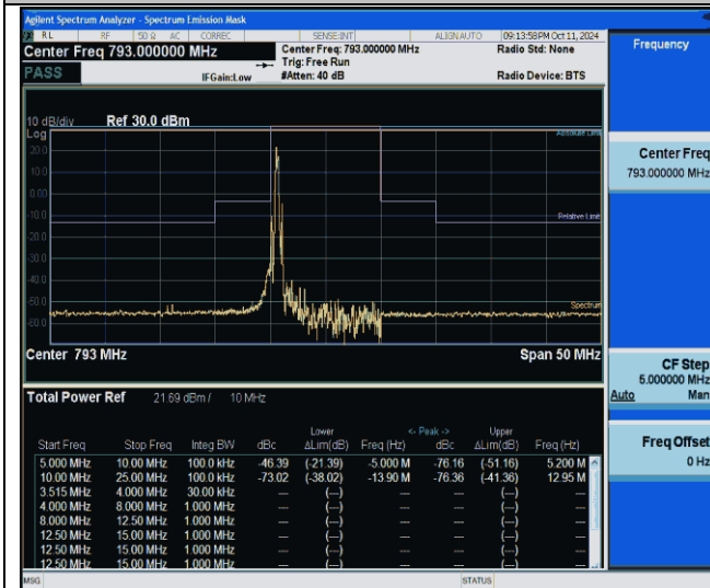
NTNV-Band14-10MHz-64QAM-23330-1RB#0-10.00-25.00-PASS
