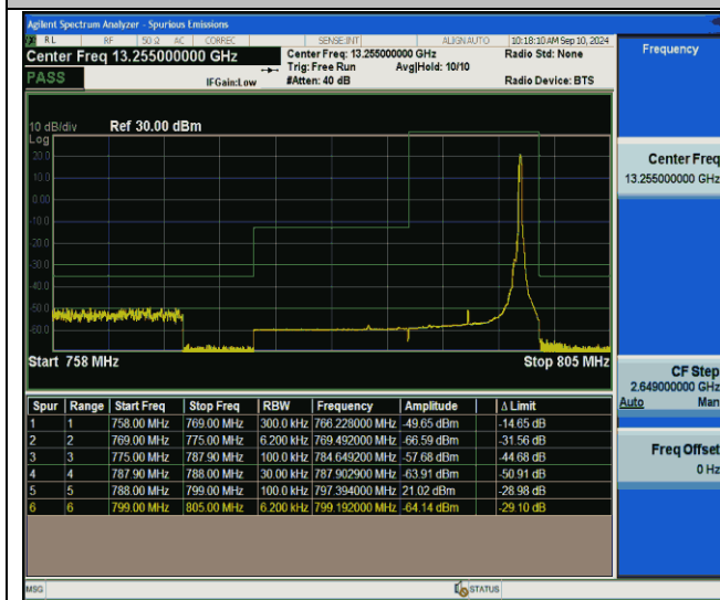
Band14-10MHz-QPSK-23330-1RB#49-PASS
