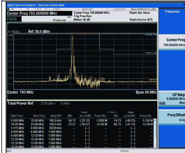
NTNV-Band14-10MHz-16QAM-23330-1RB#0-10.00-25.00-PASS
