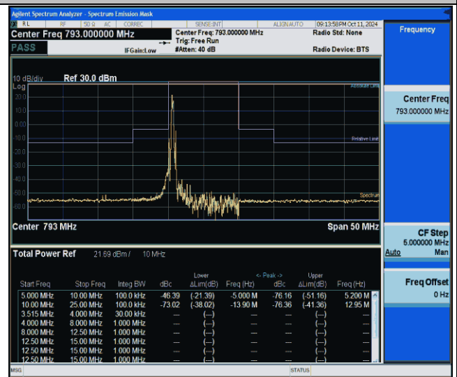
NTNV-Band14-10MHz-64QAM-23330-1RB#0-5.00-10.00-PASS
