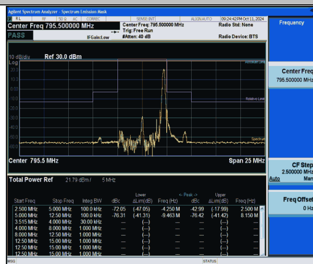
NTNV-Band14-5MHz-256QAM-23355-1RB#24--5.00--2.50-PASS
