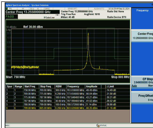
Band14-10MHz-QPSK-23330-1RB#0-PASS
