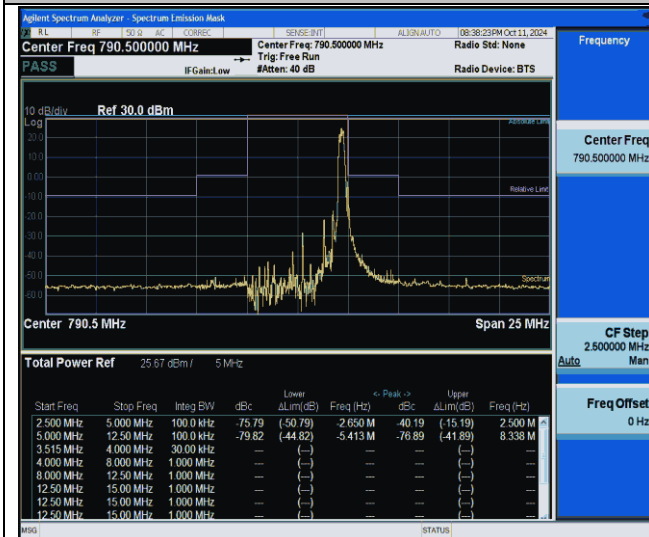
NTNV-Band14-5MHz-QPSK-23305-1RB#24--5.00--2.50-PASS
