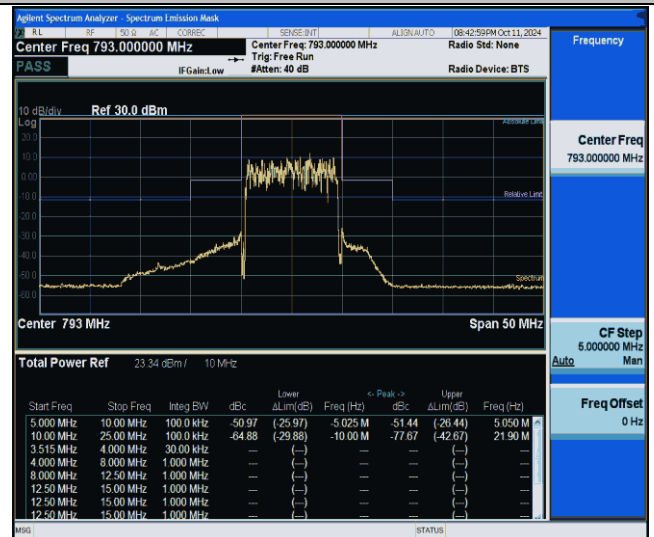
NTNV-Band14-10MHz-16QAM-23330-50RB#0--25.00--10.00-PASS
