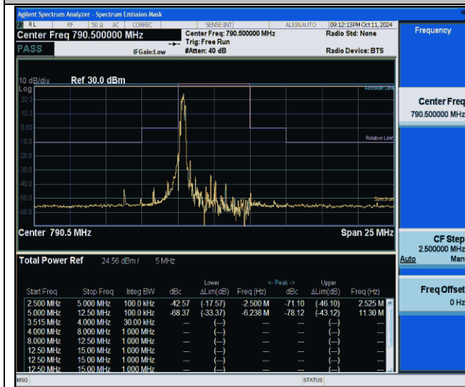
NTVN-Band14-5MHz-64QAM-23305-1RB#0-5.00-12.50-PASS
