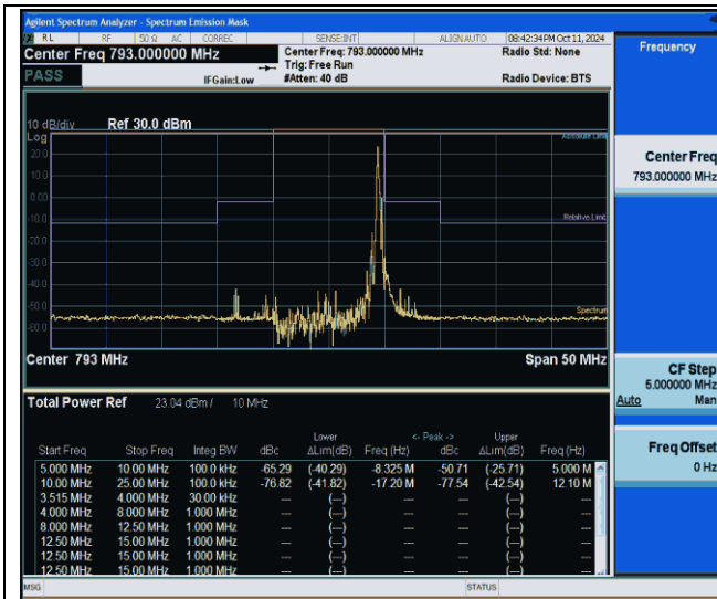
NTNV-Band14-10MHz-16QAM-23330-1RB#49-10.00-25.00-PASS
