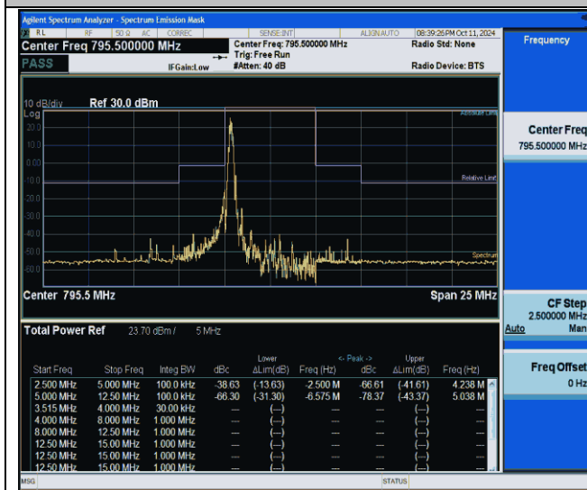
NTVN-Band14-5MHz-16QAM-23355-1RB#0--5.00--2.50-PASS
