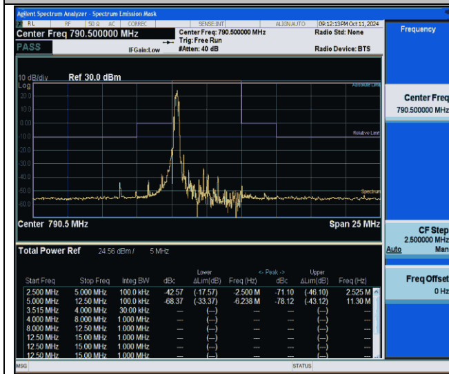
NTVN-Band14-5MHz-64QAM-23305-1RB#0--5.00--2.50-PASS
