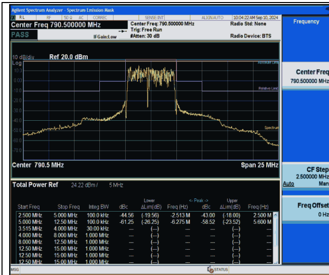
NTNV-Band14-5MHz-QPSK-23305-25RB#0--2.50-2.50-PASS
