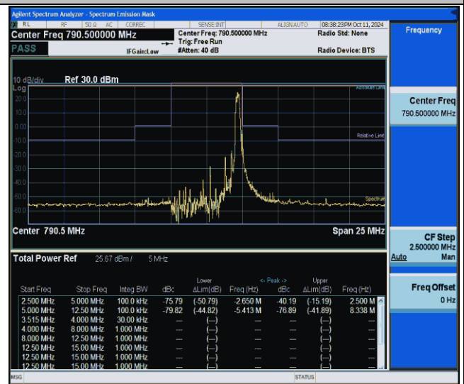
NTNV-Band14-5MHz-QPSK-23305-1RB#24--12.50--5.00-PASS
