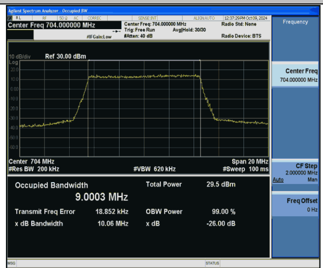
Band12-10MHz-256QAM-23060-50RB#0-PASS
