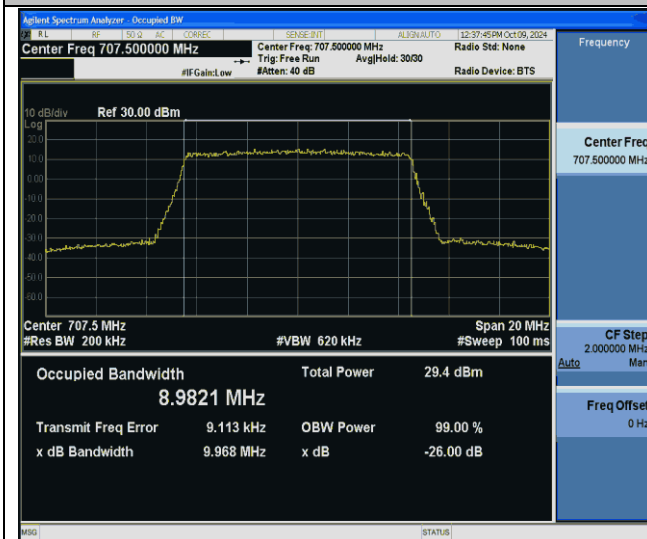
Band12-10MHz-256QAM-23095-50RB#0-PASS
