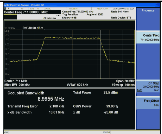
Band12-10MHz-256QAM-23130-50RB#0-PASS
