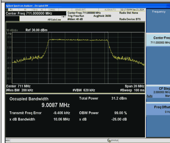
Band12-10MHz-64QAM-23130-50RB#0-PASS
