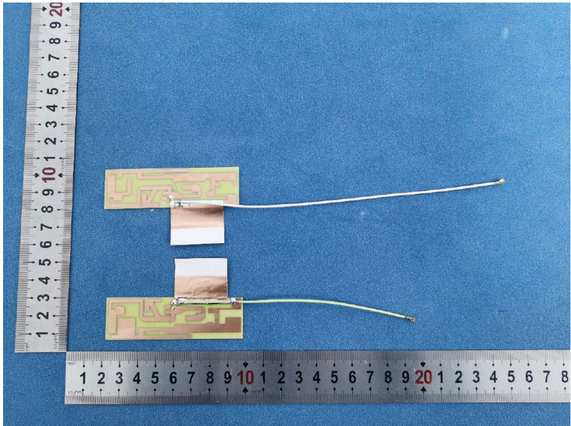
Ant1 & Ant8 (TX antenna)
