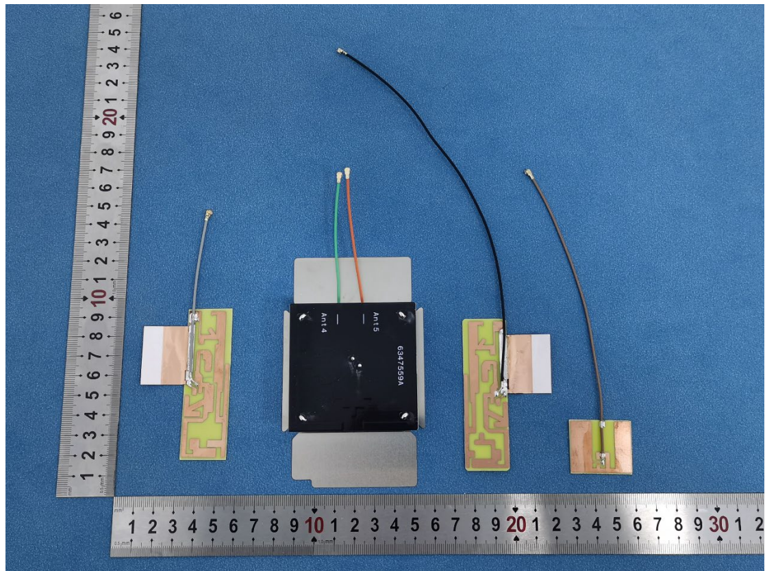
Ant3, Ant4&5, Ant6 and GPS Ant
