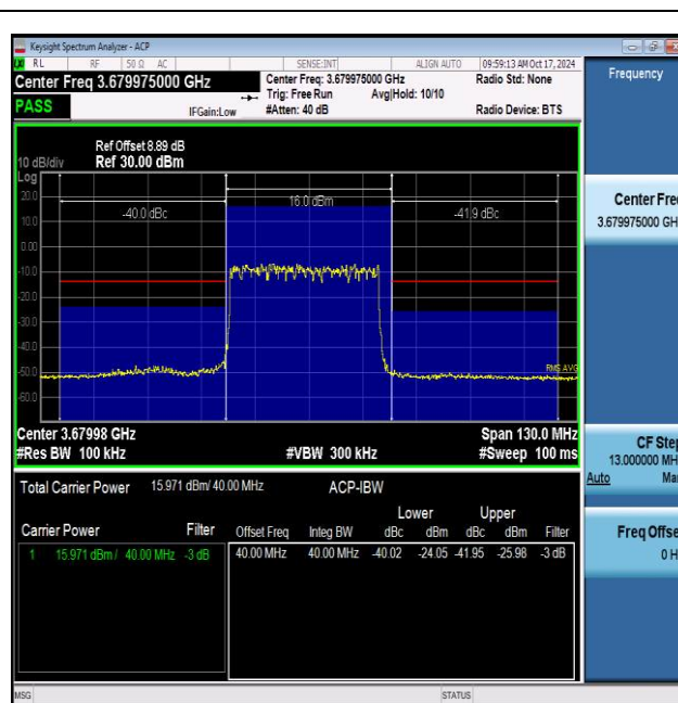
NTNV_N48_PC3_30_40_H_TID1_#1_+40_40
