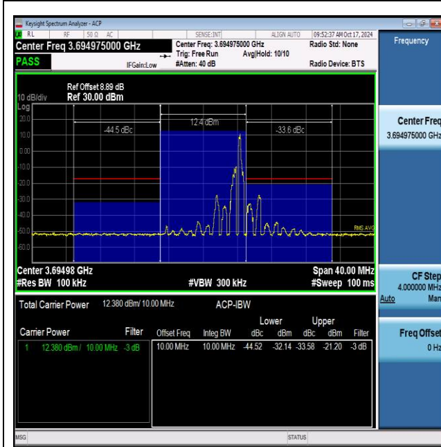
NTNV_N48_PC3_30_10_H_TID3_#1_-10_10
