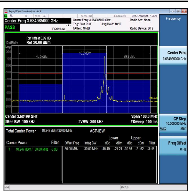
NTNV_N48_PC3_30_30_H_TID3_#1_+30_30
