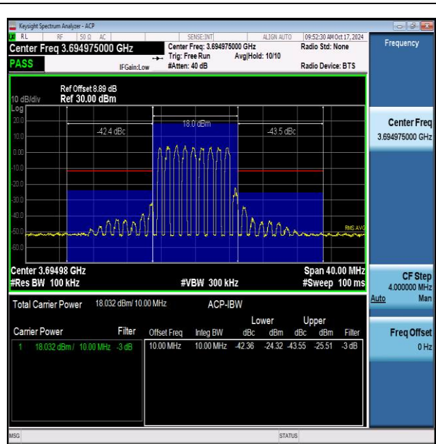
NTNV_N48_PC3_30_10_H_TID1_#1_+10_10
