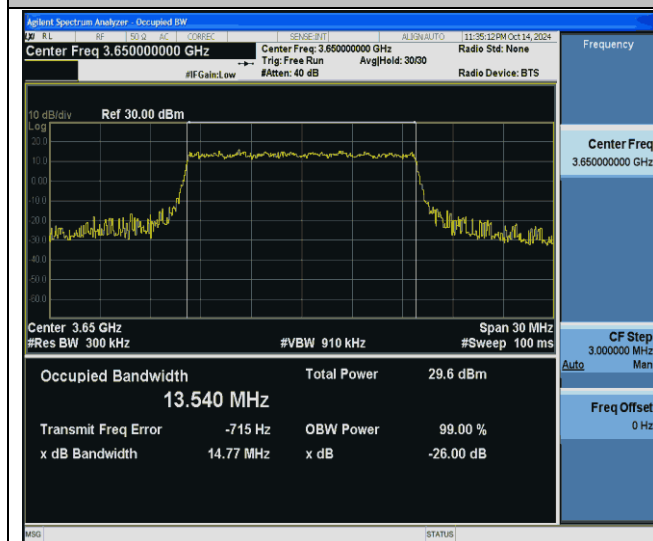
43(3600-3700)-15MHz-16QAM-44090-75RB#0-PASS
