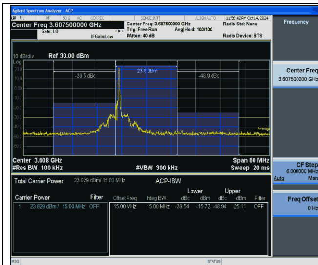
43(3600-3700)-15MHz-QPSK-43665-1RB#0-PASS
