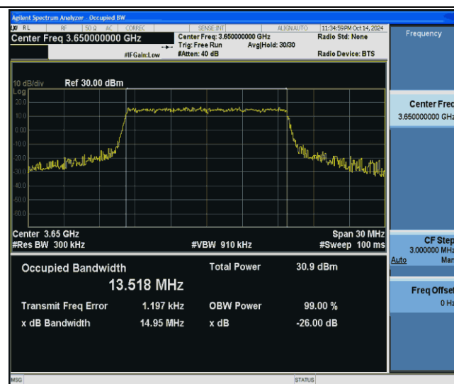
43(3600-3700)-15MHz-QPSK-44090-75RB#0-PASS
