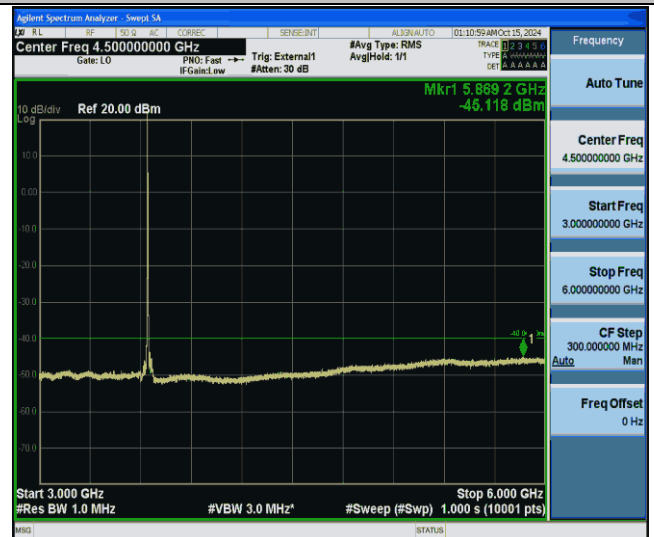
43(3600-3700)-20MHz-QPSK-44090-1RB#0-3000~6000-PASS
