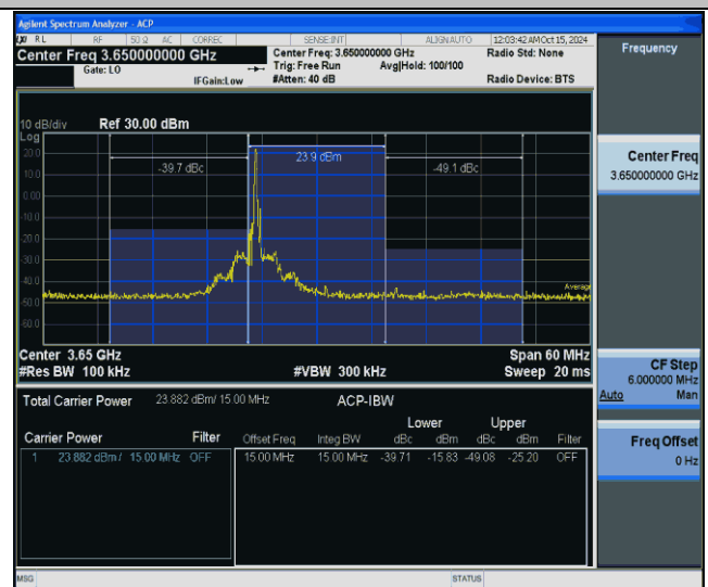
43(3600-3700)-15MHz-QPSK-44090-1RB#0-PASS
