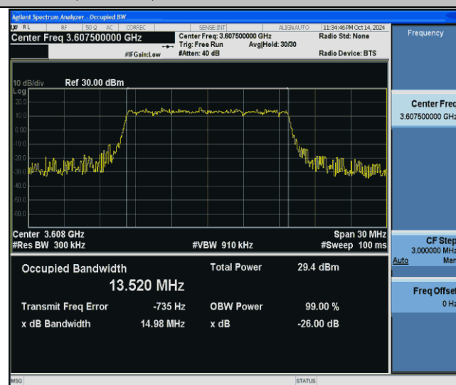
43(3600-3700)-15MHz-16QAM-43665-75RB#0-PASS
