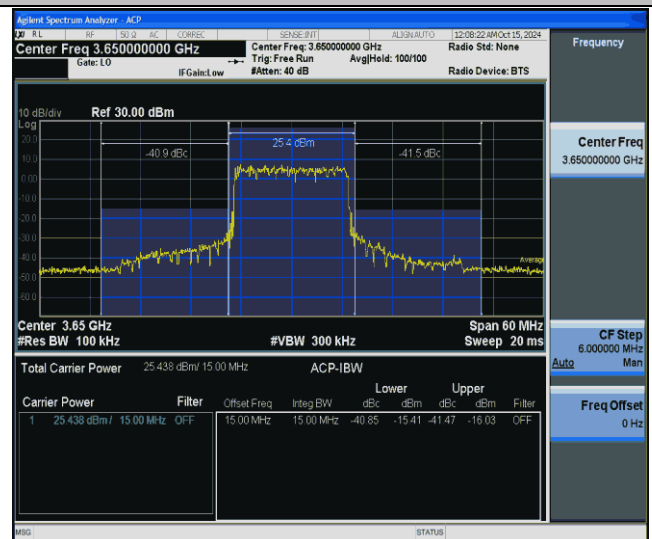
43(3600-3700)-15MHz-QPSK-44090-75RB#0-PASS
