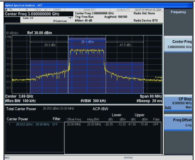
43(3600-3700)-20MHz-QPSK-44490-100RB#0-PASS
