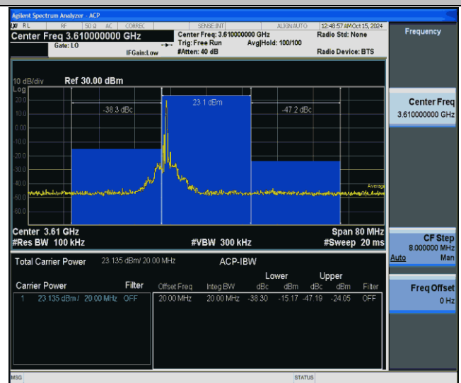
43(3600-3700)-20MHz-QPSK-43690-1RB#0-PASS
