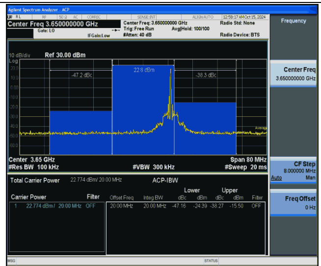
43(3600-3700)-20MHz-QPSK-44090-1RB#99-PASS
