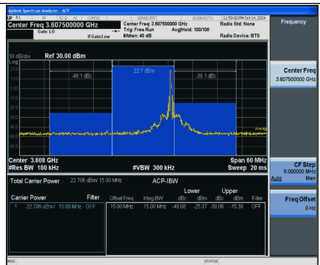
43(3600-3700)-15MHz-QPSK-43665-1RB#74-PASS
