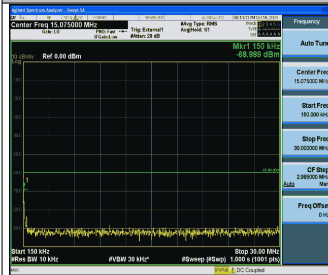
43(3600-3700)-20MHz-QPSK-44090-1RB#0-0.15~30-PASS
