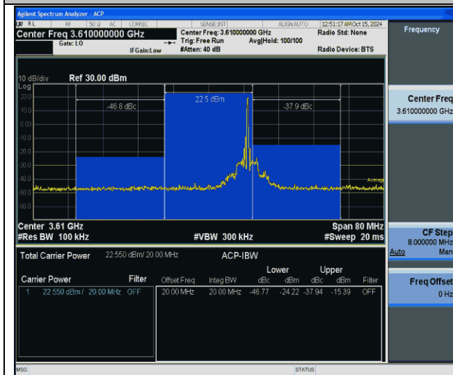
43(3600-3700)-20MHz-QPSK-43690-1RB#99-PASS
