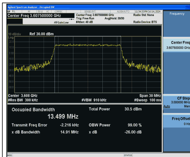
43(3600-3700)-15MHz-QPSK-43665-75RB#0-PASS
