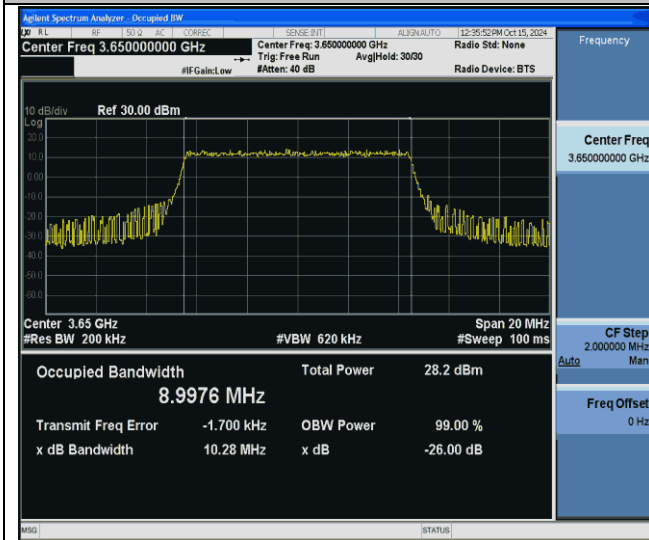
43(3600-3700)-10MHz-256QAM-44090-50RB#0-PASS
