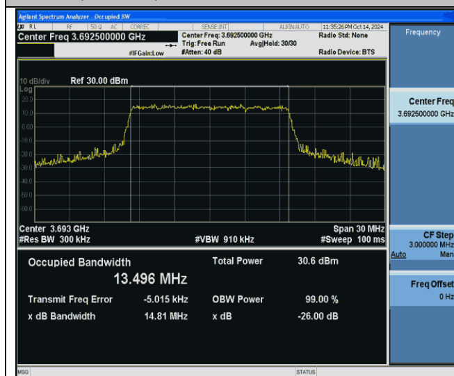
43(3600-3700)-15MHz-QPSK-44515-75RB#0-PASS
