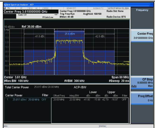
43(3600-3700)-20MHz-QPSK-43690-100RB#0-PASS
