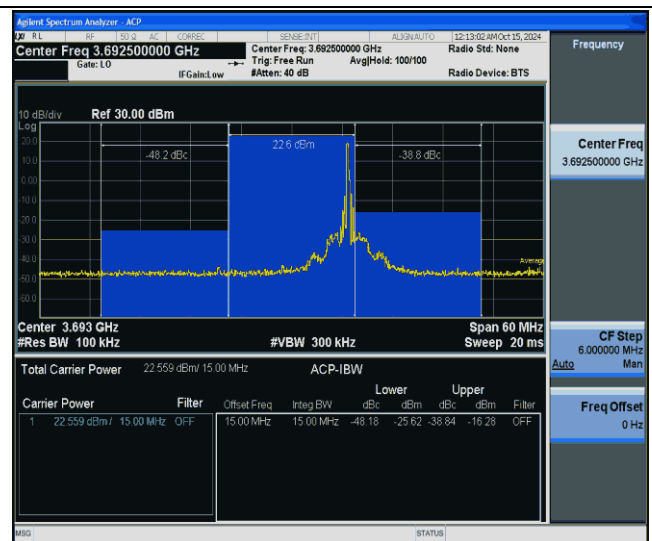
43(3600-3700)-15MHz-QPSK-44515-1RB#74-PASS
