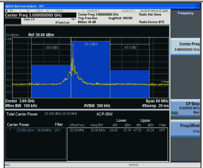
43(3600-3700)-20MHz-QPSK-44490-1RB#0-PASS
