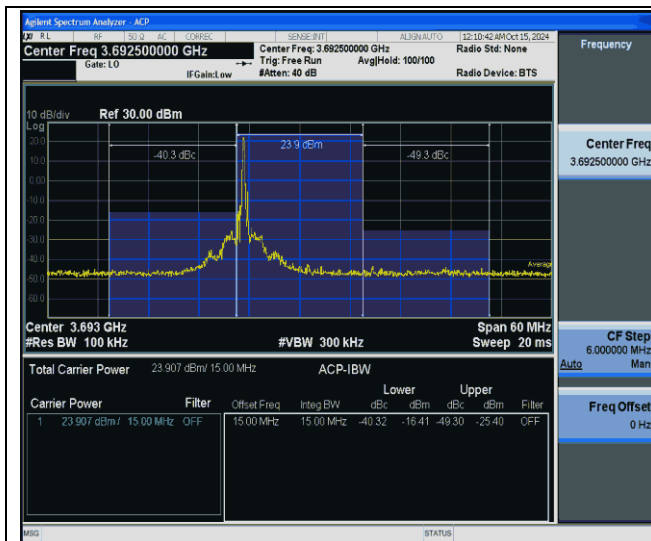
43(3600-3700)-15MHz-QPSK-44515-1RB#0-PASS
