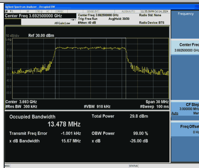
43(3600-3700)-15MHz-16QAM-44515-75RB#0-PASS
