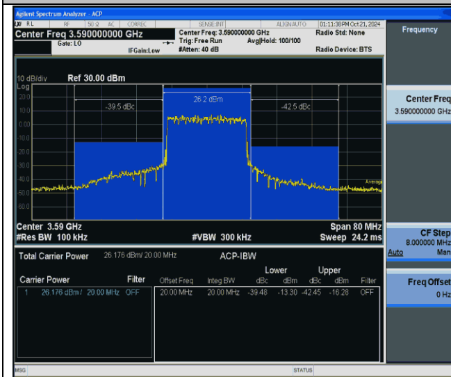
42(3550-3600)-20MHz-QPSK-43490-100RB#0-PASS
