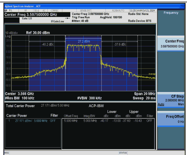
42(3550-3600)-5MHz-QPSK-43565-25RB#0-PASS
