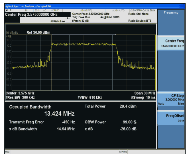
42(3550-3600)-15MHz-64QAM-43340-75RB#0-PASS
