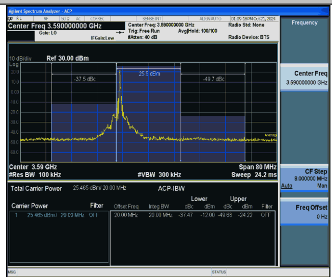
42(3550-3600)-20MHz-QPSK-43490-1RB#0-PASS
