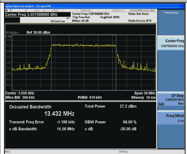
42(3550-3600)-15MHz-256QAM-43165-75RB#0-PASS
