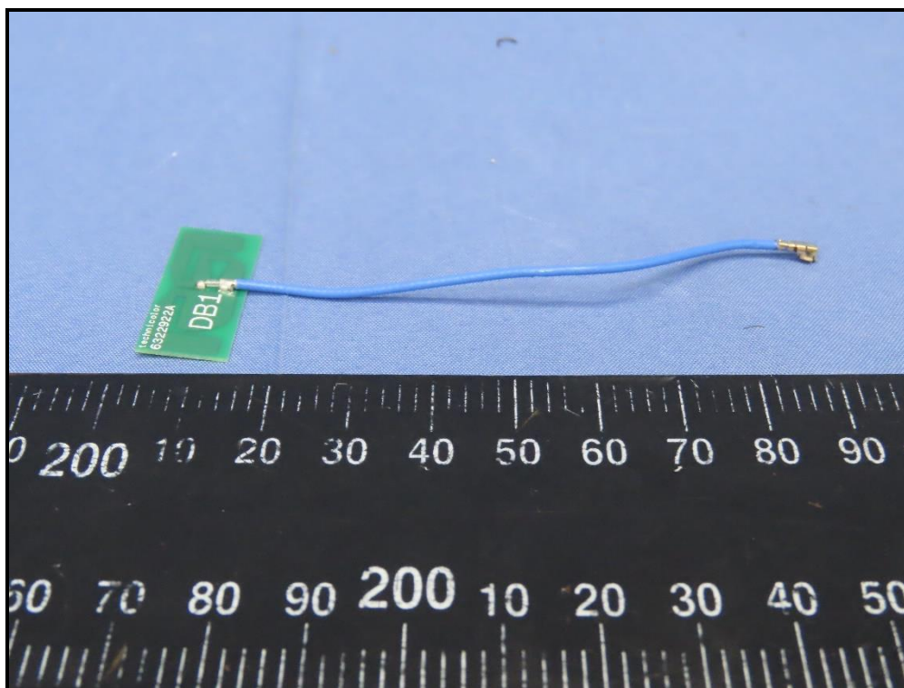
DB1 Antenna
