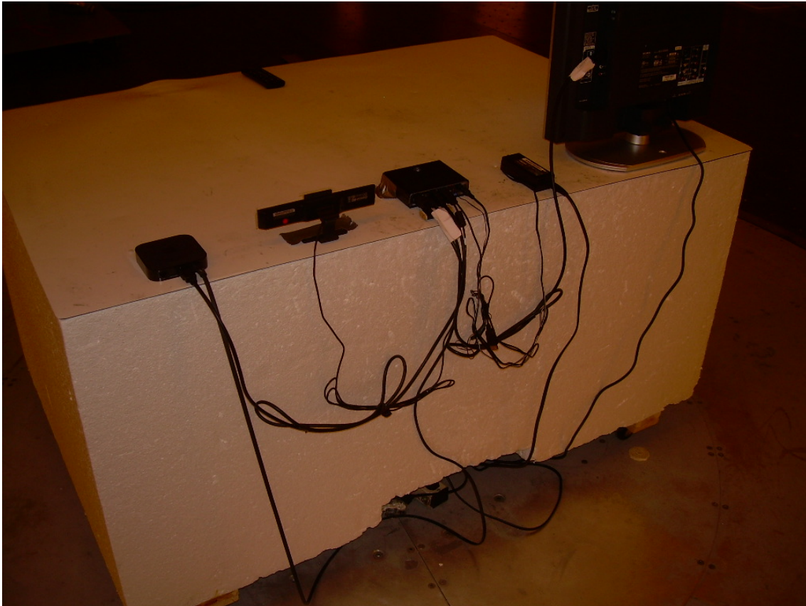
Back View Radiated Disturbance Test Configuration
