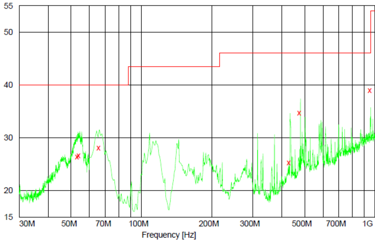
Figure 12: Spurious emission measurement results, high channel, 30-1000MHz, horizontal polarization
