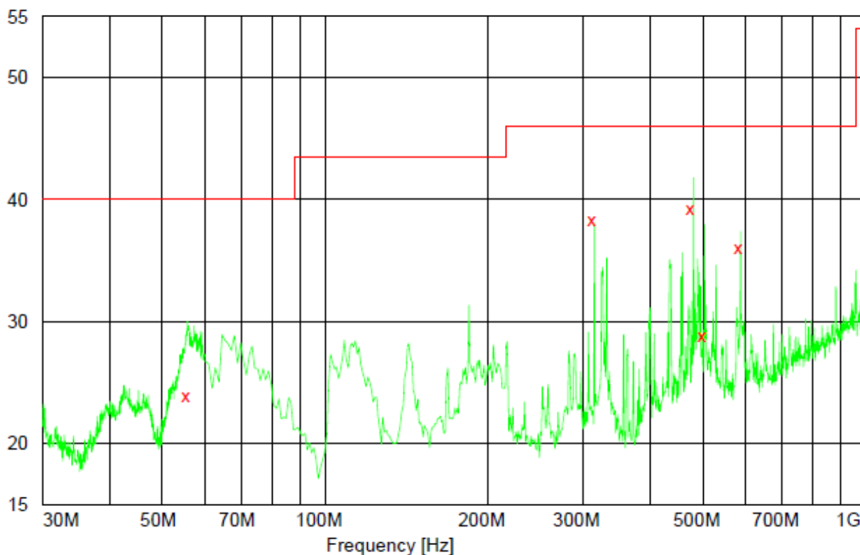
Figure 11: Spurious emission measurement results, high channel, 30-1000MHz, vertical polarization
