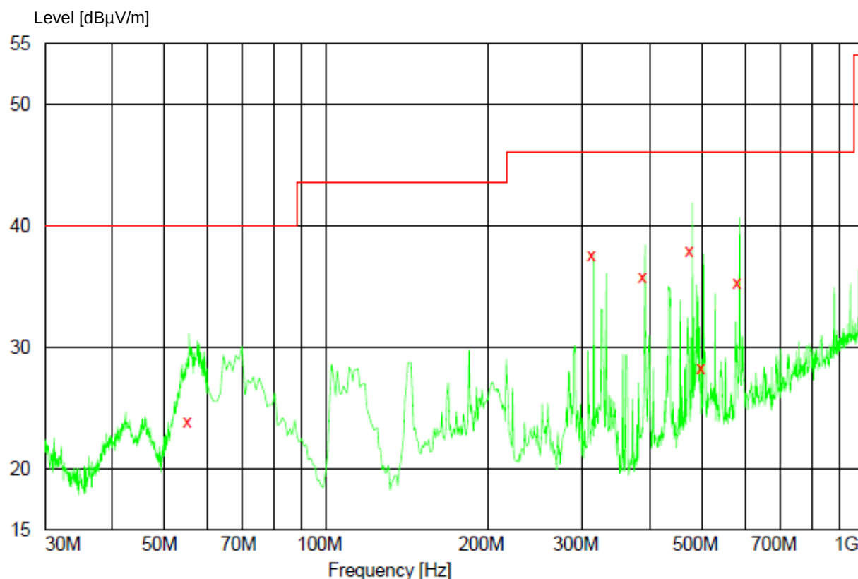
Figure 1: Spurious emission measurement results, low channel, 30-1000MHz, vertical polarization
