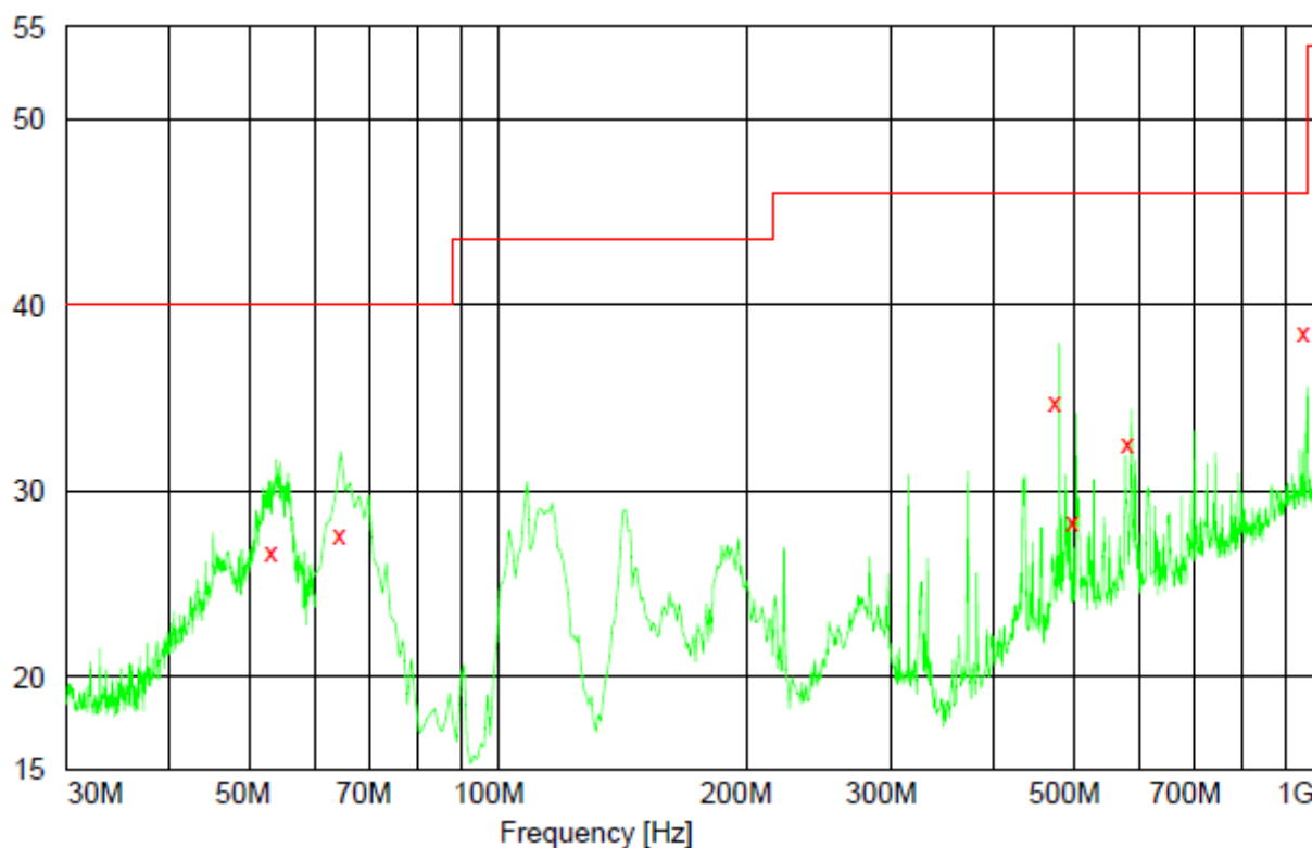
Figure 7: Spurious emission measurement results, mid channel, 30-1000MHz, horizontal polarization
