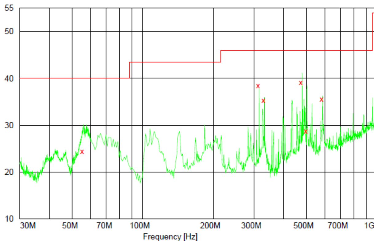
Figure 6: Spurious emission measurement results, mid channel, 30-1000MHz, vertical polarization
