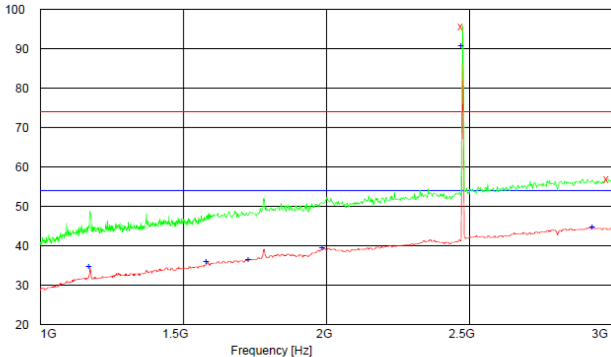
Figure 13: Spurious emission measurement results, high channel, 1-3GHz, vertical and horizontal polarization
