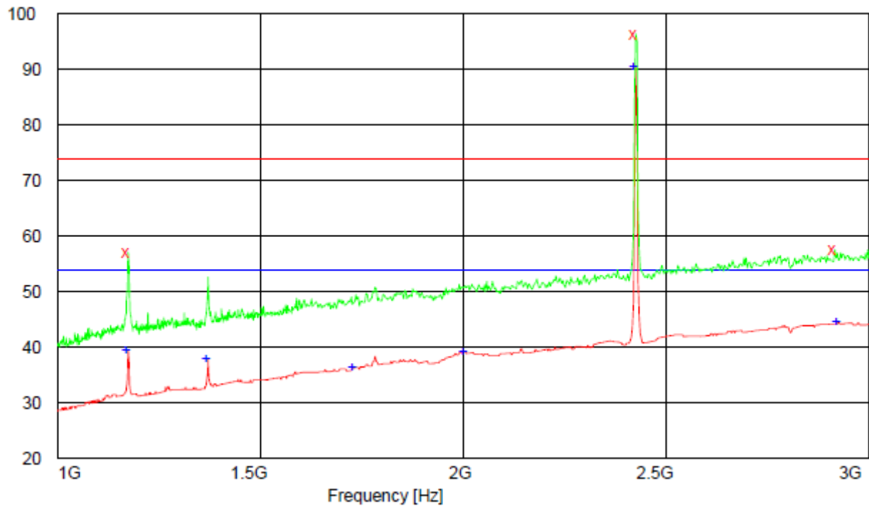
Figure 3: Spurious emission measurement results, low channel, 1-3GHz, vertical and horizontal polarization
