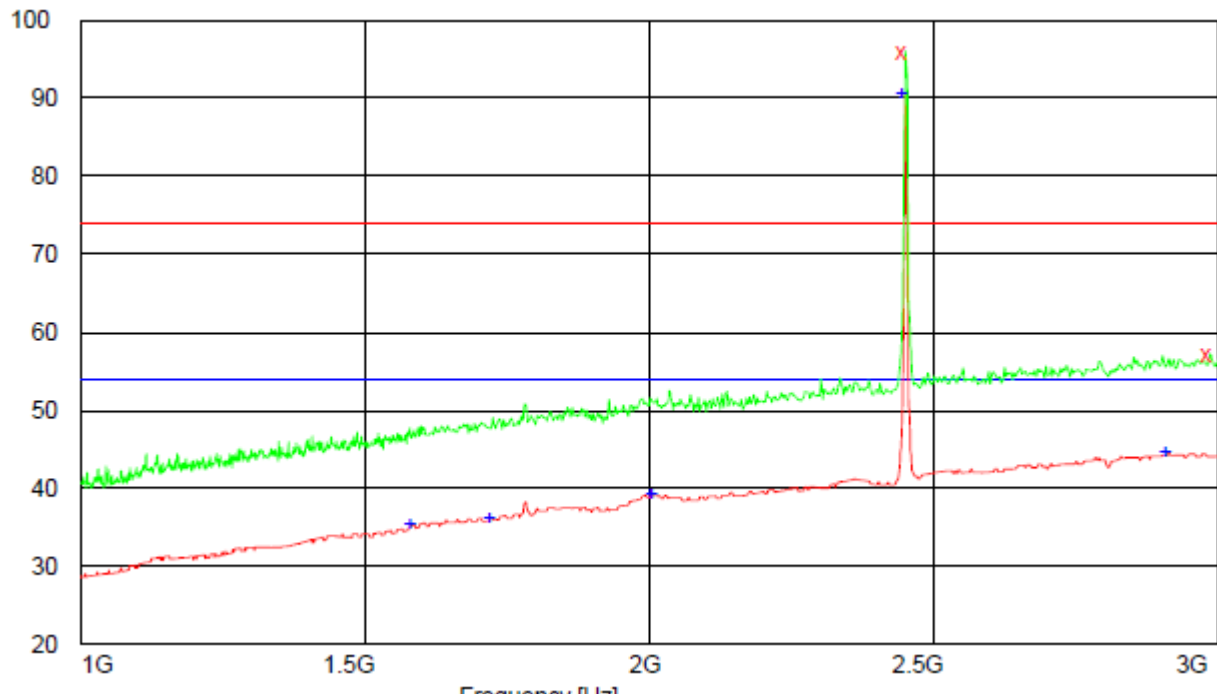
Figure 8: Spurious emission measurement results, mid channel, 1-3GHz, vertical and horizontal polarization
