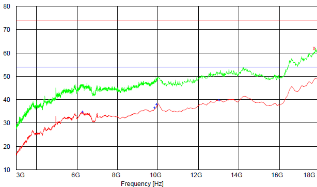
Figure 14: Spurious emission measurement results, high channel, 3-18GHz, vertical and horizontal polarization
