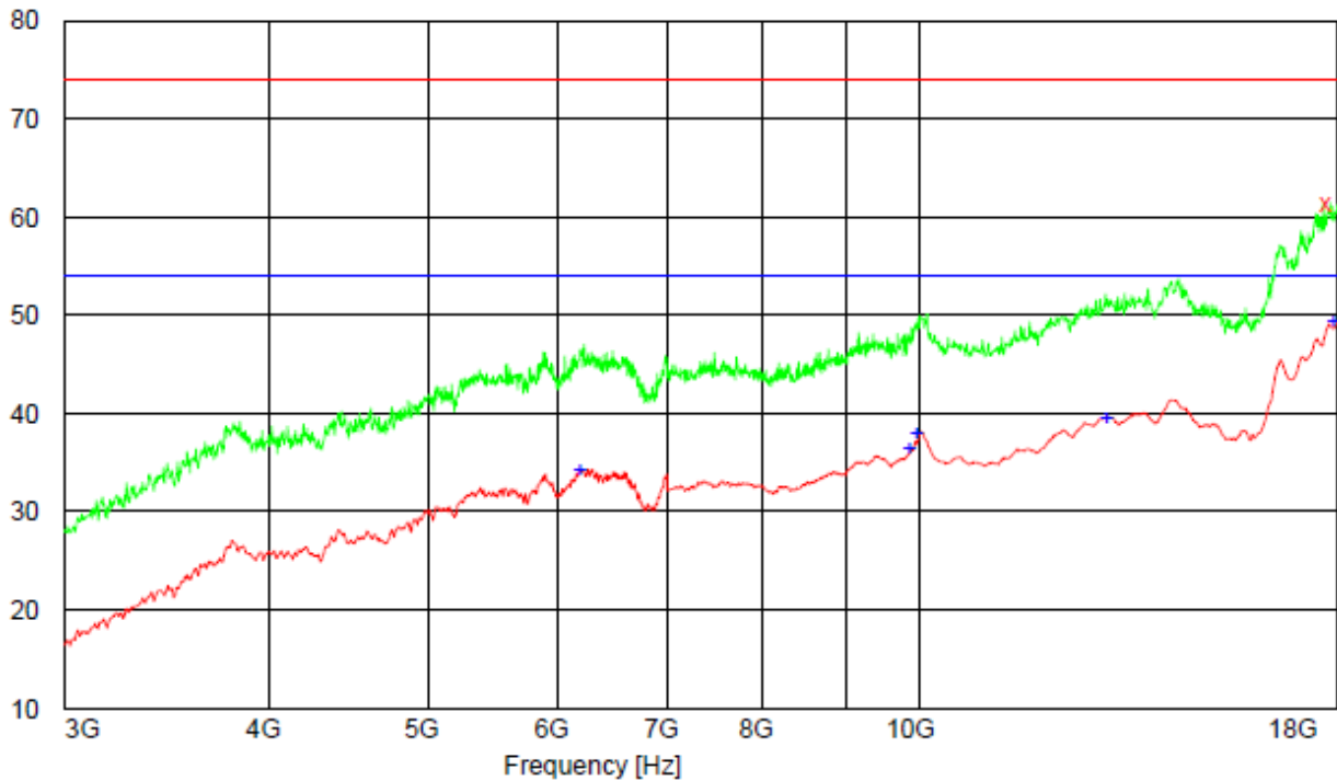
Figure 9: Spurious emission measurement results, mid channel, 3-18GHz, vertical and horizontal polarization
