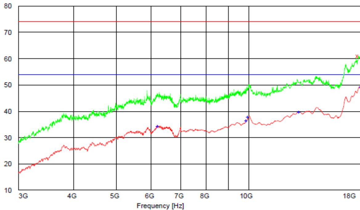
Figure 4: Spurious emission measurement results, low channel, 3-18GHz, vertical and horizontal polarization
