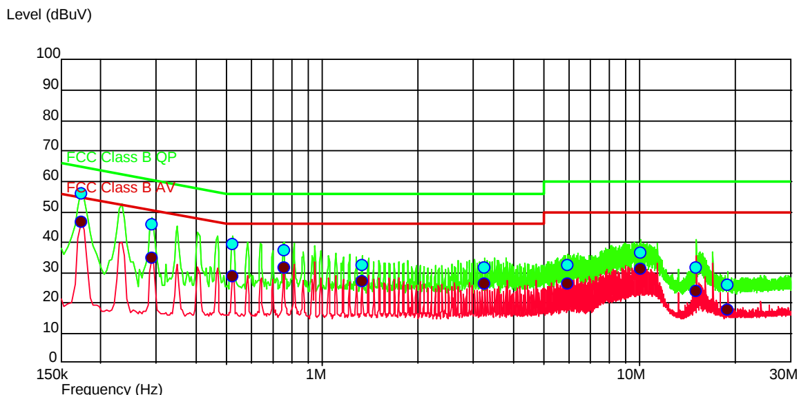
Figure 17: Conducted emission measurement results, Line L
