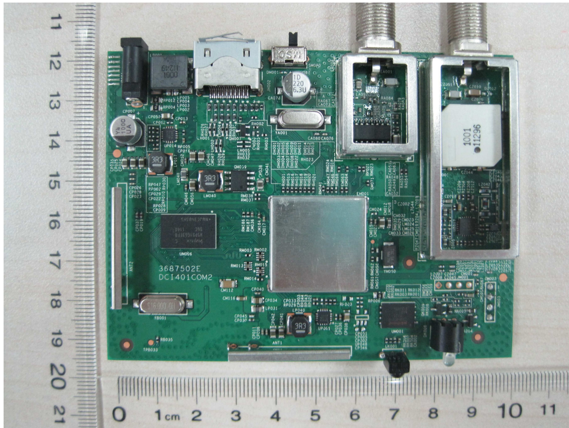
Pic5: PCB component side (with shielding) of DCI401COM2
