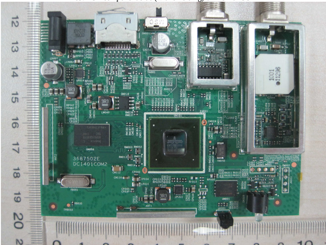
Pic6: PCB component side (without shielding) of DCI401COM2
