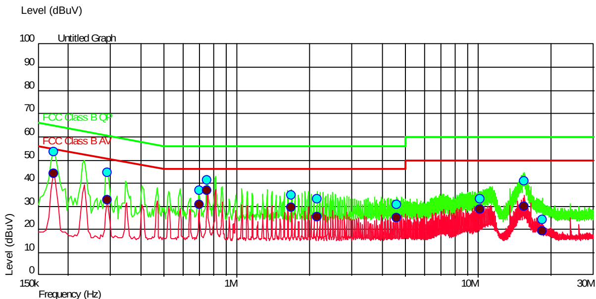
Figure 4: Conducted emission measurement results, Line N
