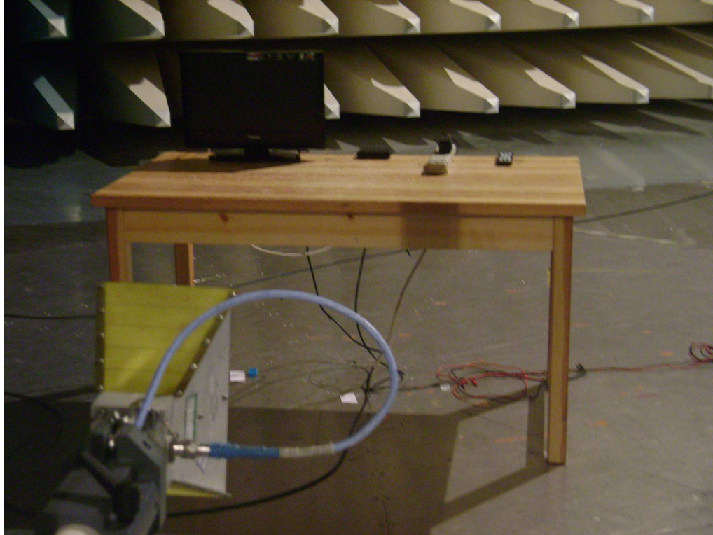
Photograph 3: Set-up for Radiated Emissions 1GHz – 2GHz
