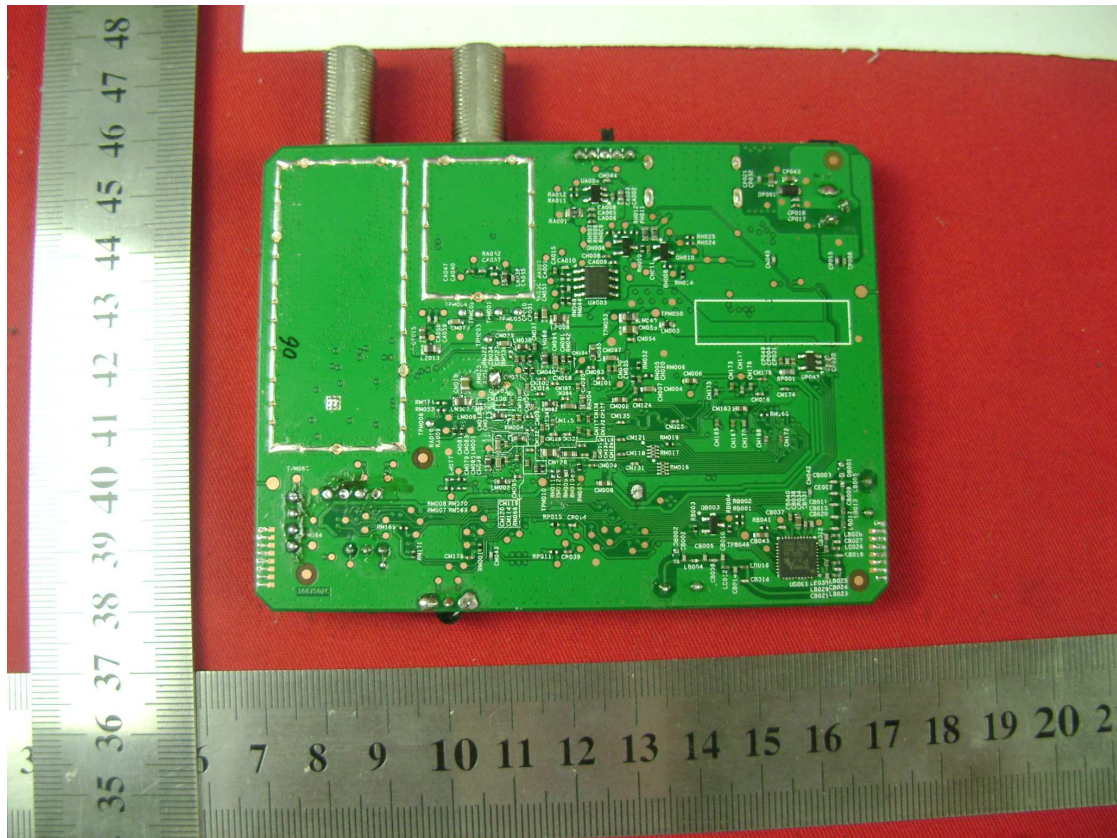
Pic7: PCB trace side of DCI401COM2
