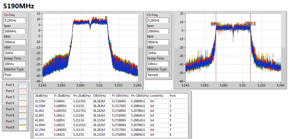
802.11ac VHT40-BF_Nss1,(MCS0)_8TX
