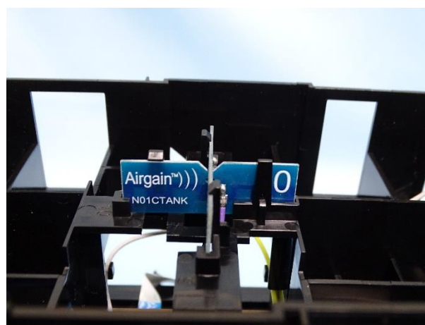
Fig.10 Antenna #10 (ZIGBEE)
