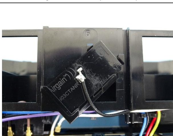
Fig.6 Antenna #6 (WLAN 2.4G/5G)
