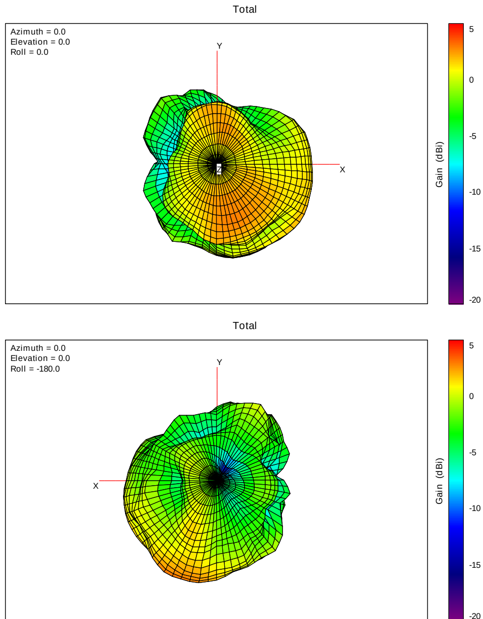
3D Free Space Gain Pattern
