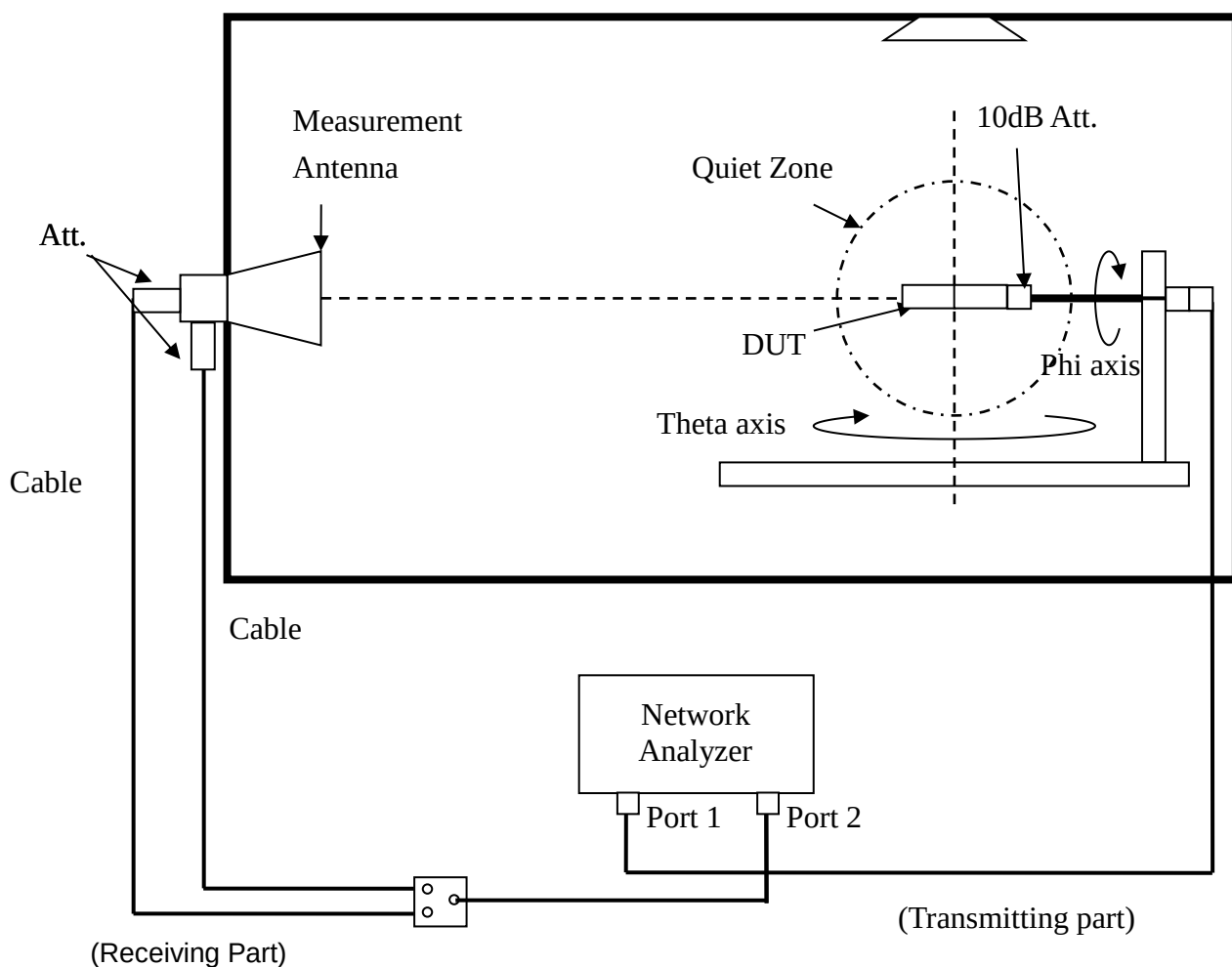
Setup of the passive Measurement
