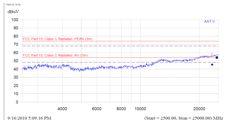
(Plot C.7: Antenna Vertical, 2.5GHz to 25GHz)
