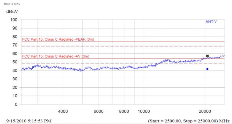
(Plot A.7: Antenna Vertical, 2.5GHz to 25GHz)
