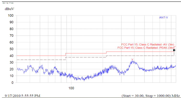
(Plot C.5: Antenna Vertical, 30MHz to 1GHz)
