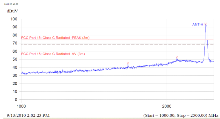
(Plot A.3: Antenna Horizontal, 1GHz to 2.5GHz)
