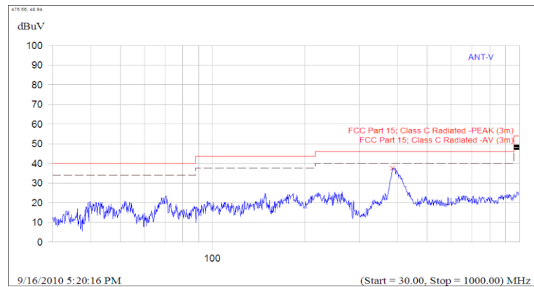
(Plot C.5: Antenna Vertical, 30MHz to 1GHz)
