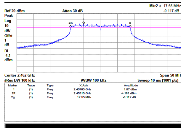
(Plot C: Channel 11: 2462MHz)
