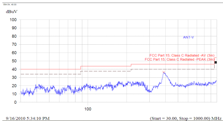
(Plot B.5: Antenna Vertical, 30MHz to 1GHz)
