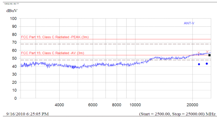
(Plot A.7: Antenna Vertical, 2.5GHz to 25GHz)
