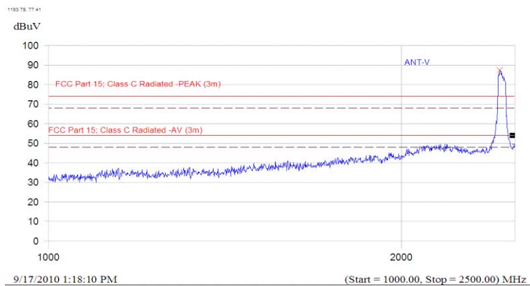
(Plot B.6: Antenna Vertical, 1GHz to 2.5GHz)
