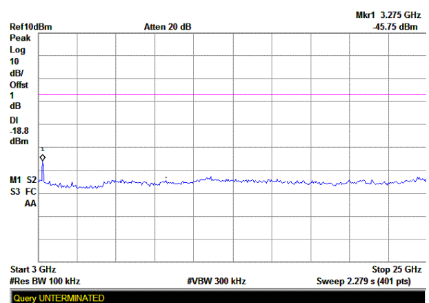
(Plot A.2: Channel = 1, 3GHz to 25GHz)
