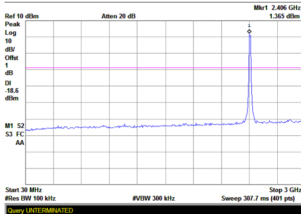
(Plot A.1: Channel = 1, 30MHz to 3GHz)
