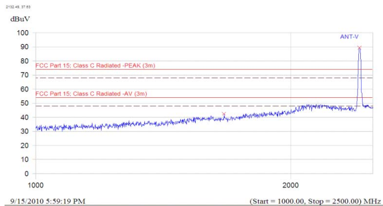
(Plot A.6: Antenna Vertical, 1GHz to 2.5GHz)
