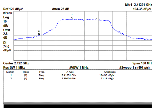
(Plot A1: Channel = 3 PEAK)
