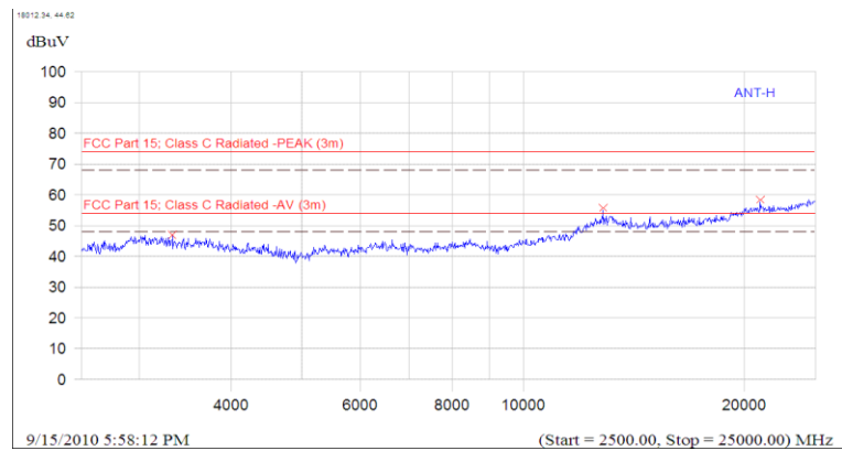
(Plot B.4: Antenna Horizontal, 2.5GHz to 25GHz)
