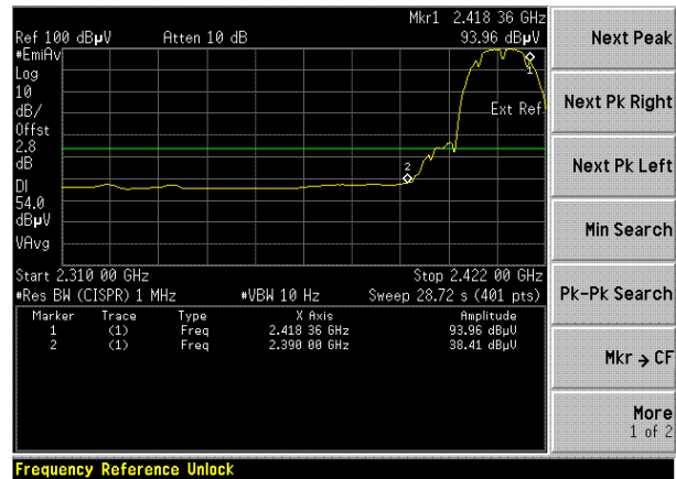
(Plot A2: Channel = 1 AVG)
