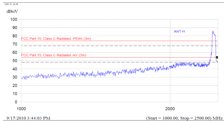
(Plot C.3: Antenna Horizontal, 1GHz to 2.5GHz)
