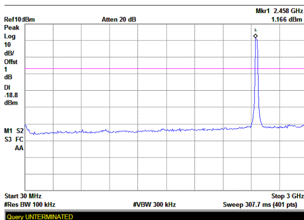
(Plot A.1: Channel = 1, 30MHz to 3GHz)
