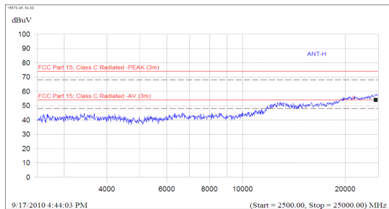
(Plot C.4: Antenna Horizontal, 2.5GHz to 25GHz)
