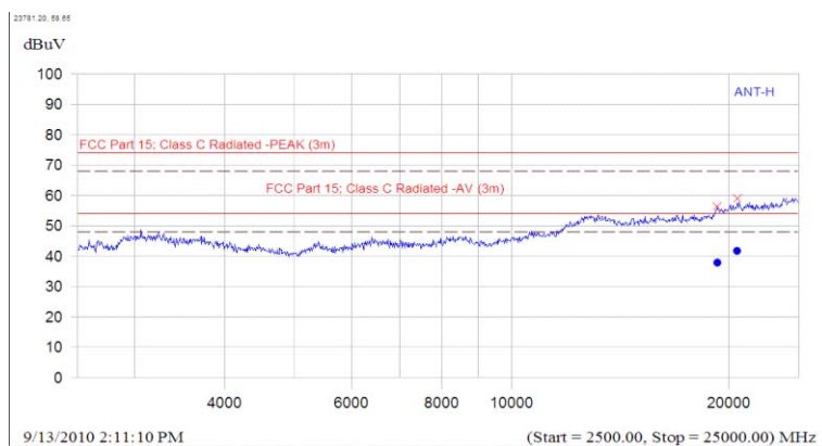
(Plot B.4: Antenna Horizontal, 2.5GHz to 25GHz)
