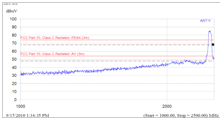
(Plot C.6: Antenna Vertical, 1GHz to 2.5GHz)
