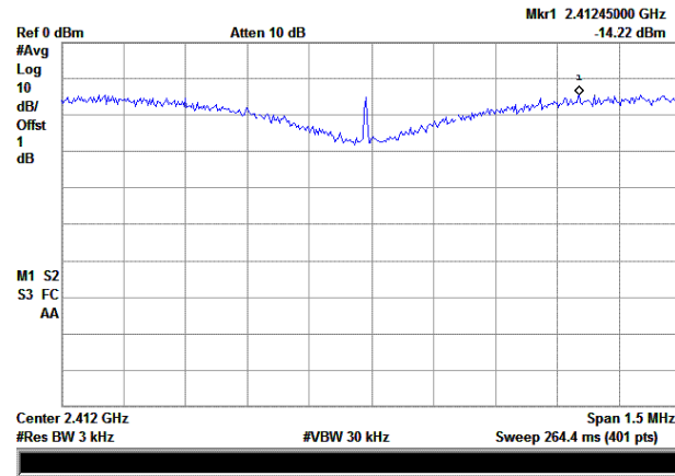
(Plot A: Channel = 1)
