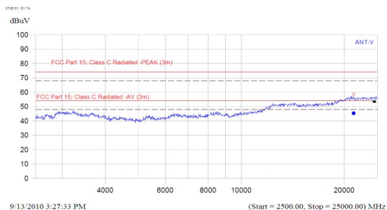
(Plot C.7: Antenna Vertical, 2.5GHz to 25GHz)
