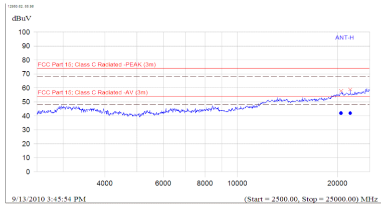
(Plot C.4: Antenna Horizontal, 2.5GHz to 25GHz)
