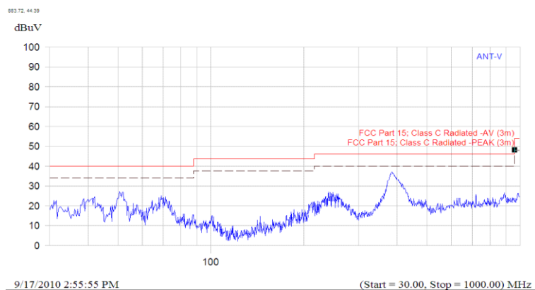
(Plot A.5: Antenna Vertical, 30MHz to 1GHz)
