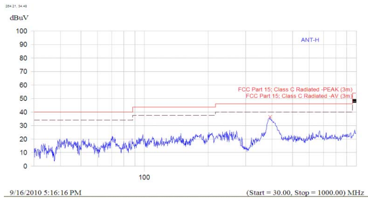
(Plot C.2: Antenna Horizontal, 30MHz to 1GHz)
