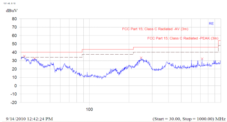
(Plot A.2: Antenna Horizontal, 30MHz to 1GHz)
