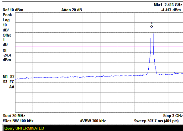
(Plot A.1: Channel = 3, 30MHz to 3GHz)
