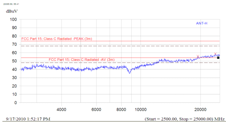
(Plot A.4: Antenna Horizontal, 2.5GHz to 25GHz)
