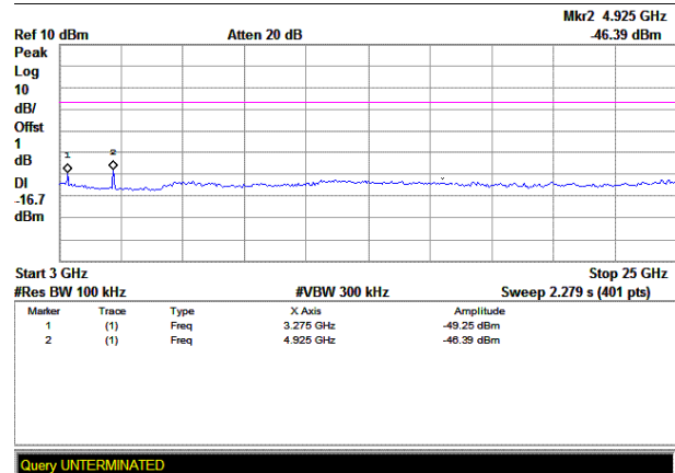
(Plot C.2: Channel = 11, 3GHz to 25GHz)
