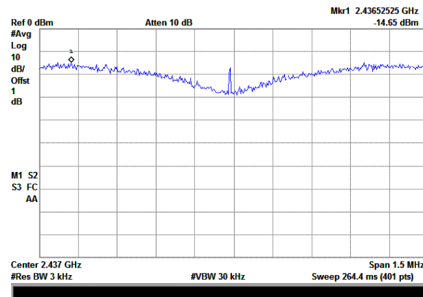
(Plot B: Channel = 6)
