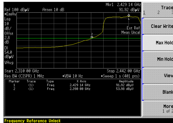
(Plot A2: Channel = 3 AVG)
