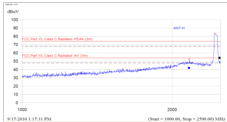
(Plot B.3: Antenna Horizontal, 1GHz to 2.5GHz)
