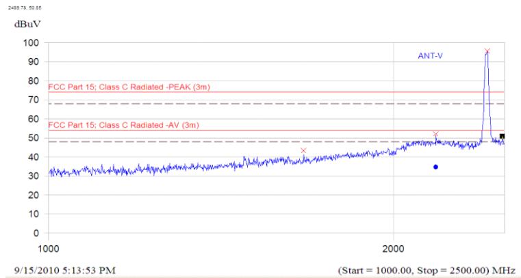
(Plot A.6: Antenna Vertical, 1GHz to 2.5GHz)
