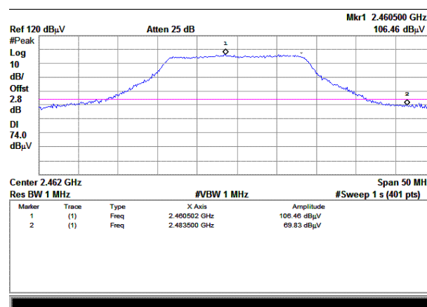
(Plot B1: Channel = 11 PEAK)
