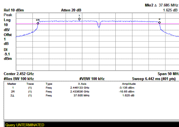
(Plot C: Channel 9: 2452MHz)
