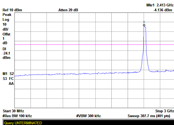
(Plot C.1: Channel = 9, 30MHz to 3GHz)
