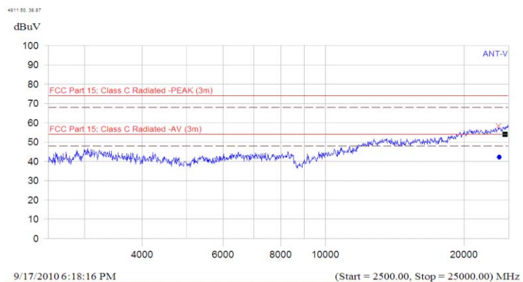
(Plot B.7: Antenna Vertical, 2.5GHz to 25GHz)
