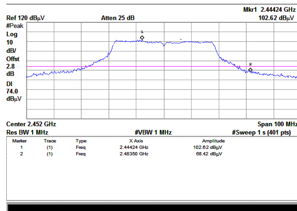
(Plot B1: Channel = 9 PEAK)
