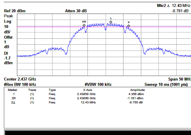
(Plot B: Channel 6: 2437 MHz)
