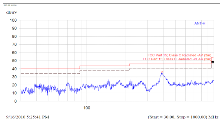
(Plot B.2: Antenna Horizontal, 30MHz to 1GHz)
