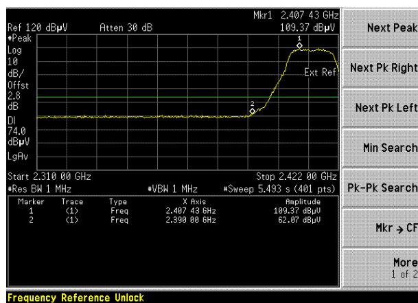
(Plot A1: Channel = 1 PEAK)
