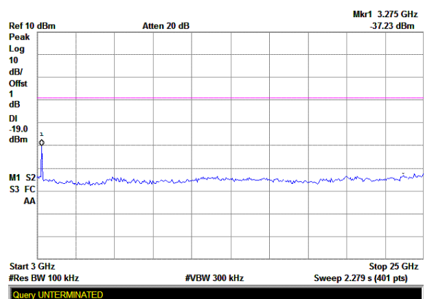
(Plot B.2: Channel = 6, 3GHz to 25GHz)
