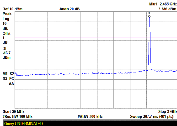
(Plot C.1: Channel = 11, 30MHz to 3GHz)
