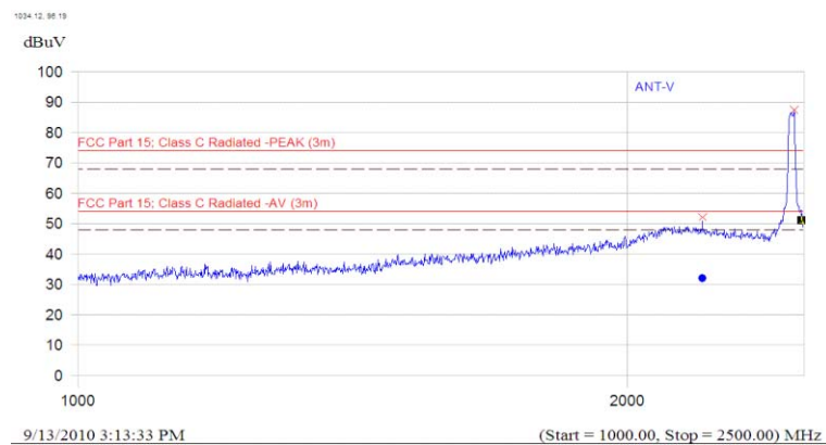
(Plot C.6: Antenna Vertical, 1GHz to 2.5GHz)
