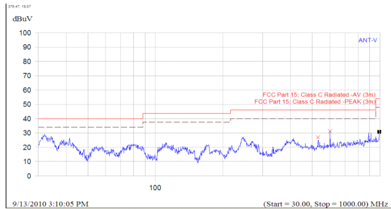
(Plot B.5: Antenna Vertical, 30MHz to 1GHz)
