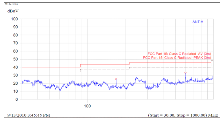
(Plot C.2: Antenna Horizontal, 30MHz to 1GHz)
