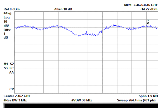
(Plot I: Channel = 11)
