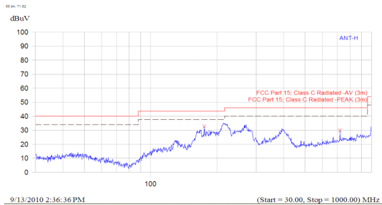
(Plot B.2: Antenna Horizontal, 30MHz to 1GHz)
