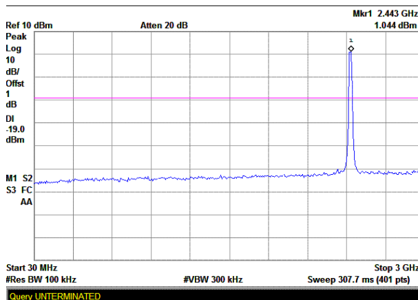
(Plot B.1: Channel = 6, 30MHz to 3GHz)
