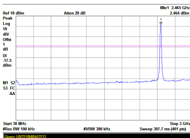
(Plot C.1: Channel = 11, 30MHz to 3GHz)
