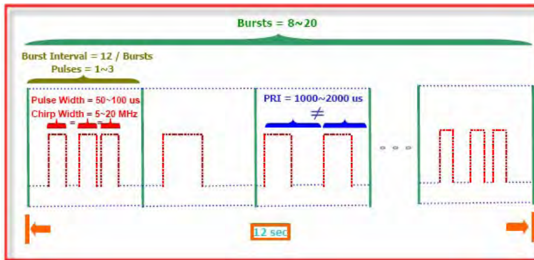
Radar Types (5) System Diagram
