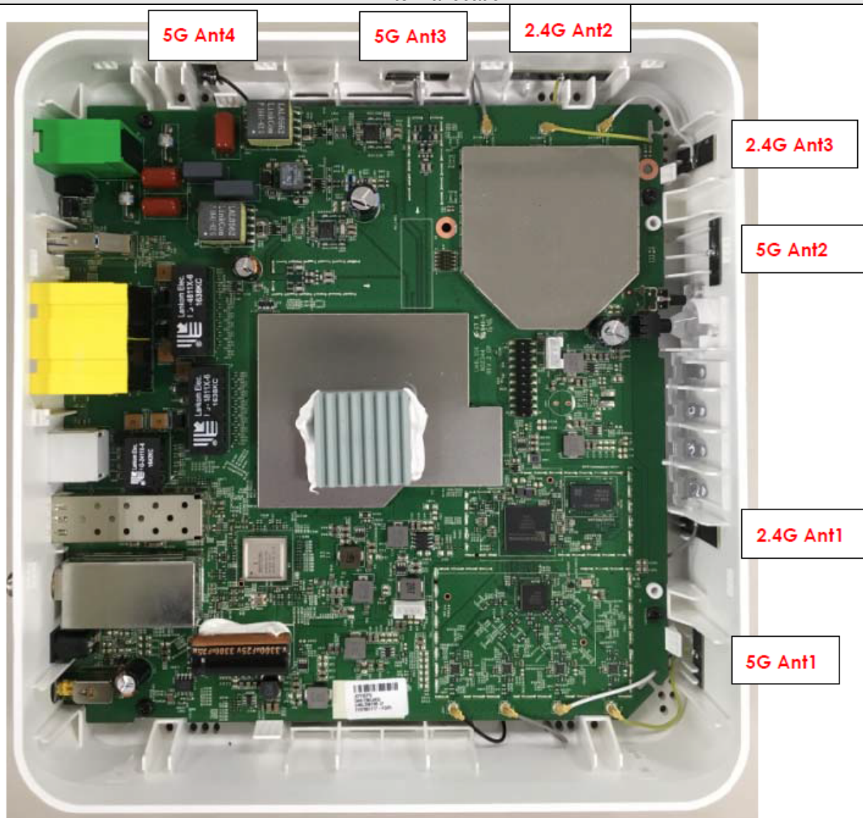
Antenna location
