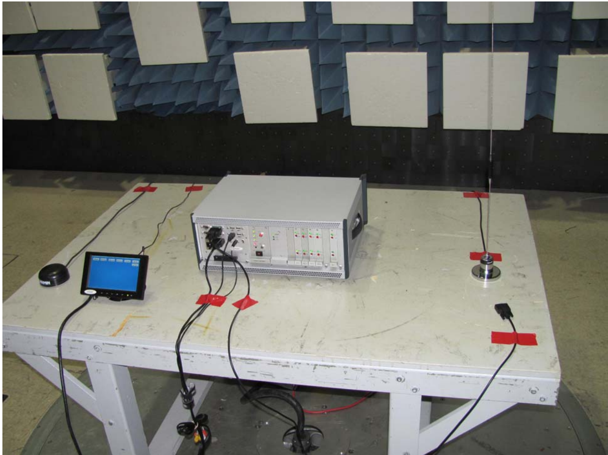
Figure 1: Internal View w/ Remote External Antenna Connection
