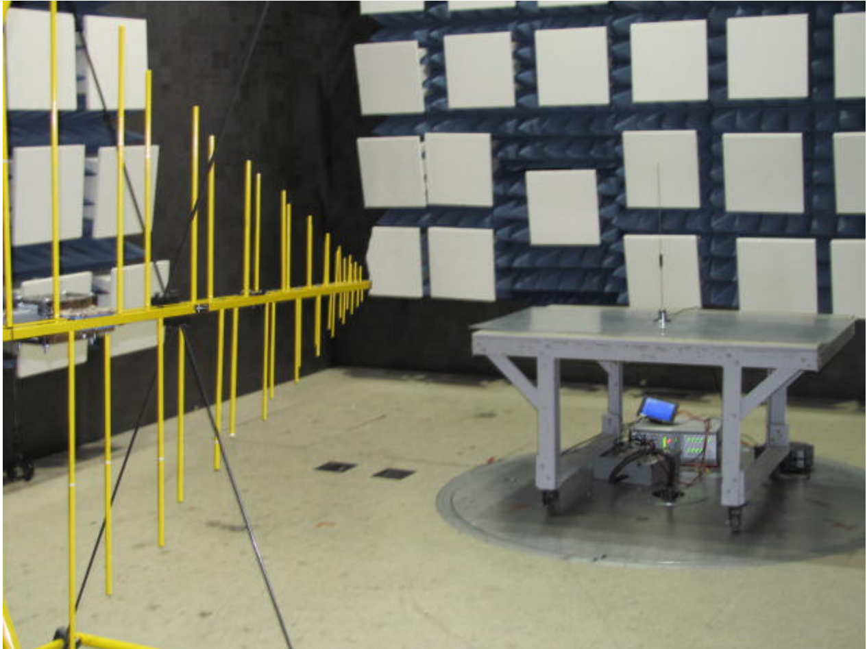
Internal view – Internal Antenna Configuration
