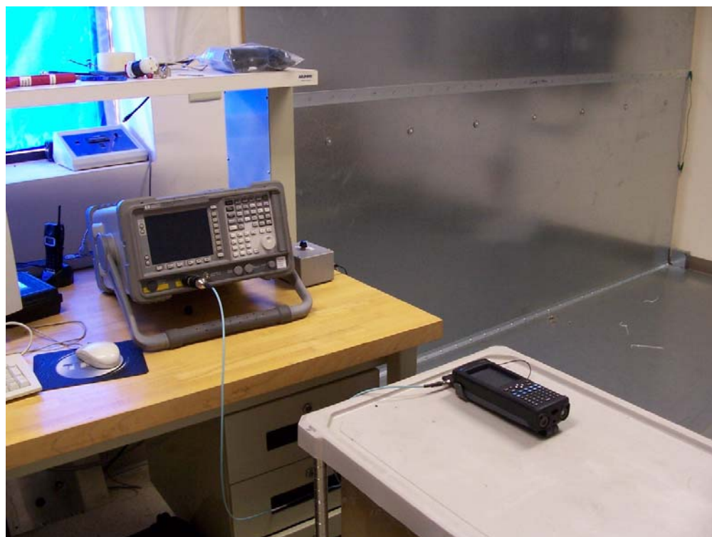
Figure 2: Additional 15.247 Antenna Port Measurements
