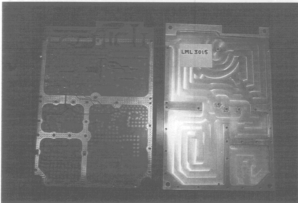
8-9 Alveolate mechanical system
