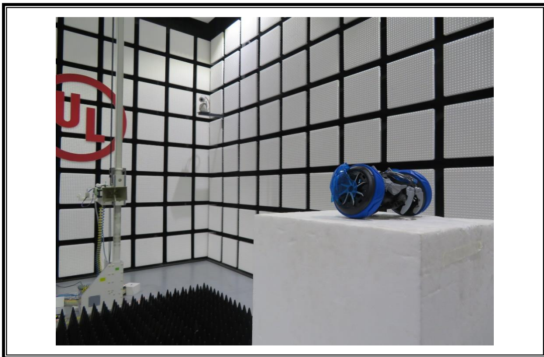
RADIATED RF MEASUREMENT SETUP (Above 1G – X axis)
