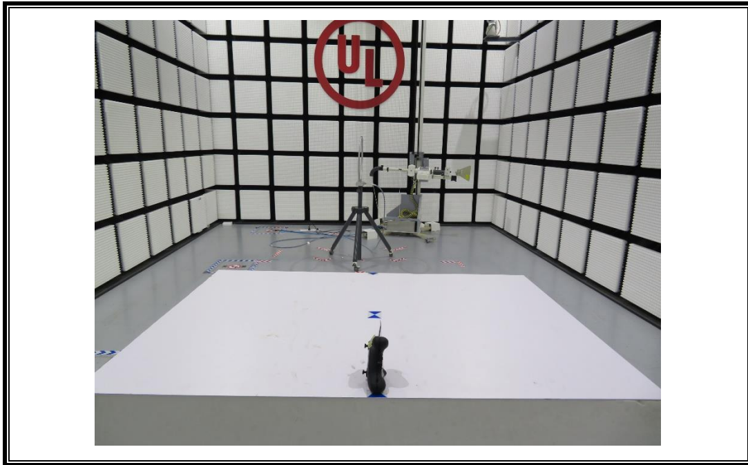
RADIATED RF MEASUREMENT SETUP (Below 30MHz – Z axis)
