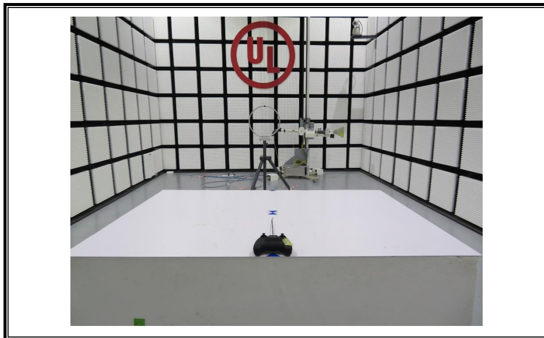
RADIATED RF MEASUREMENT SETUP (Below 30MHz– X axis)
