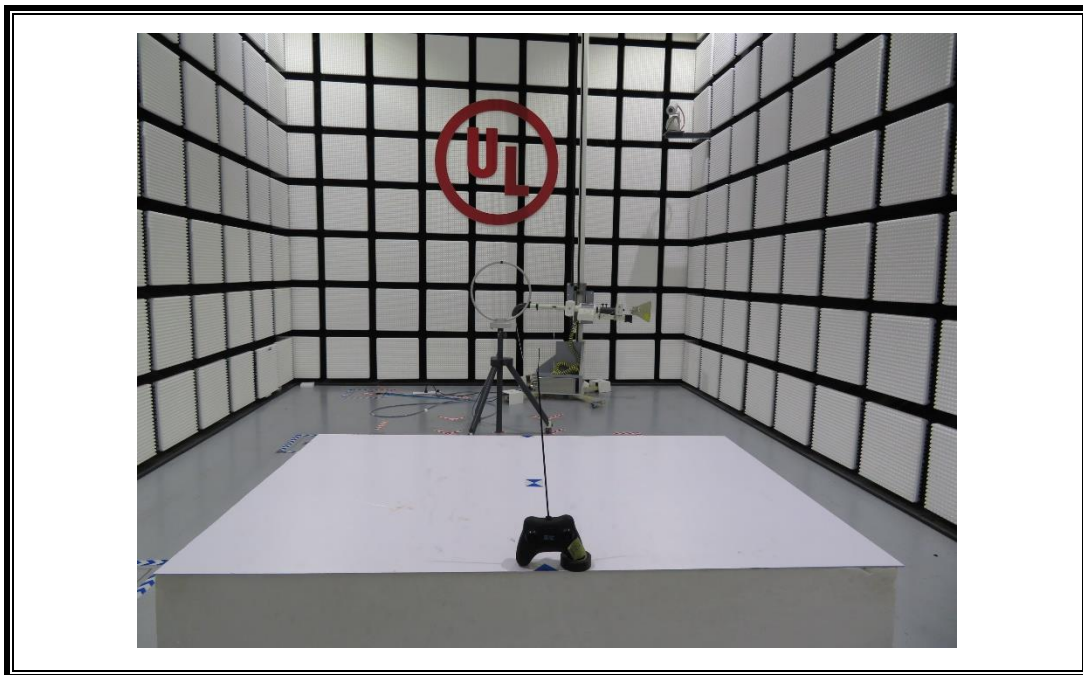
RADIATED RF MEASUREMENT SETUP (Below 30MHz – Z axis)
