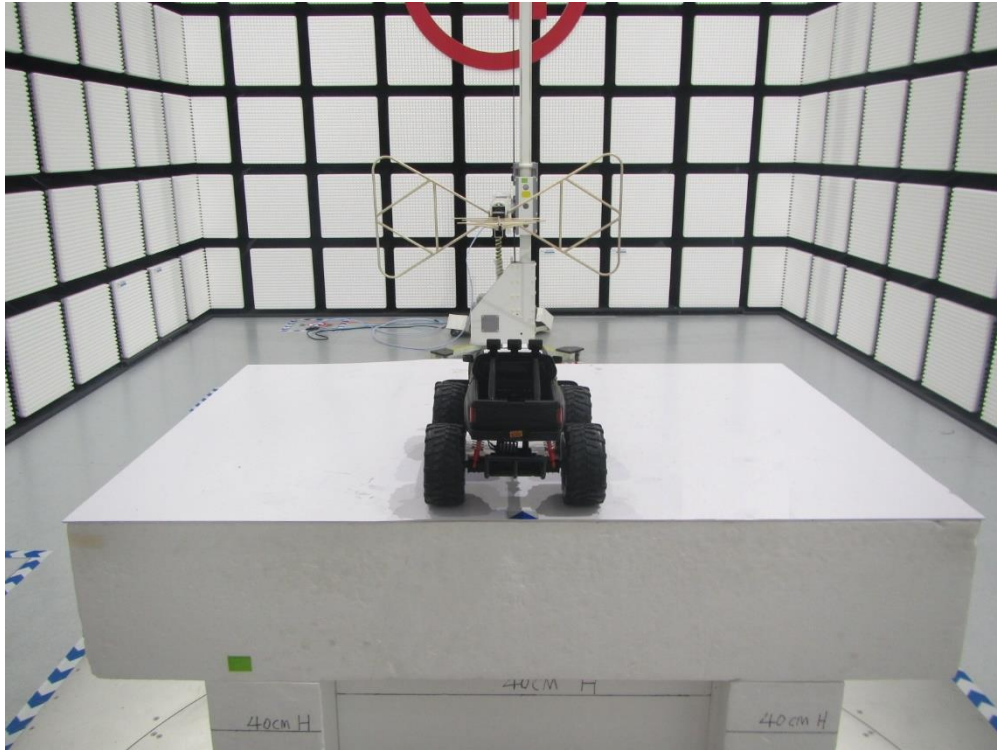
Radiated Emissions above 1GHz test setup photo
