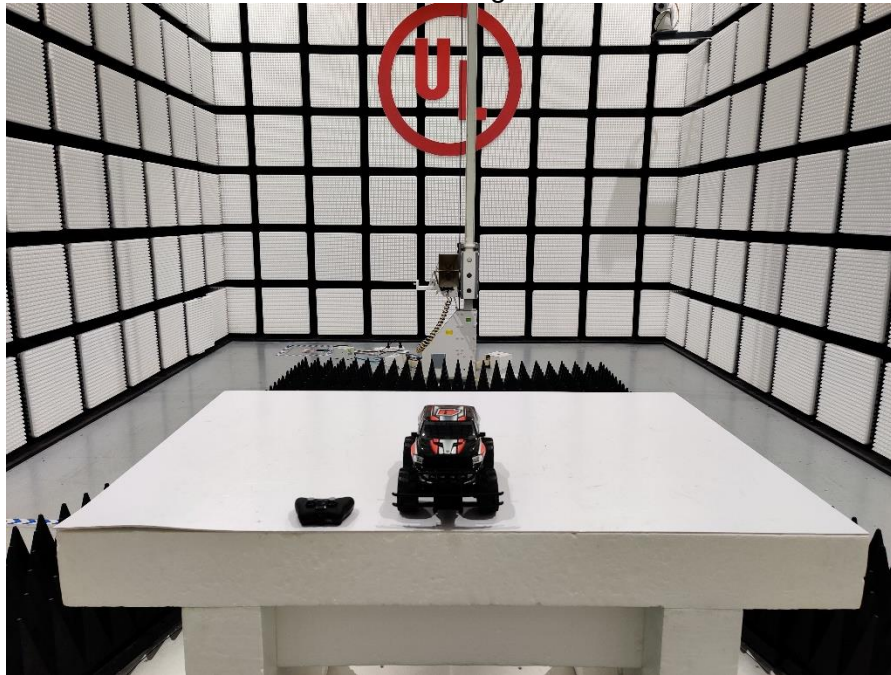
Radiated Emissions above 1GHz test setup photo
