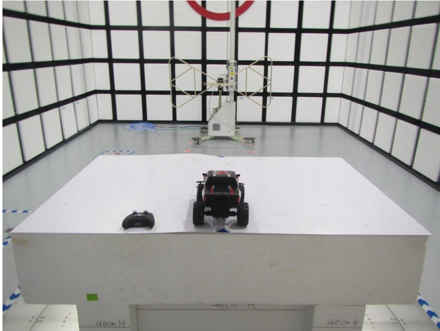
Radiated Emissions below 1GHz test setup photo Running
