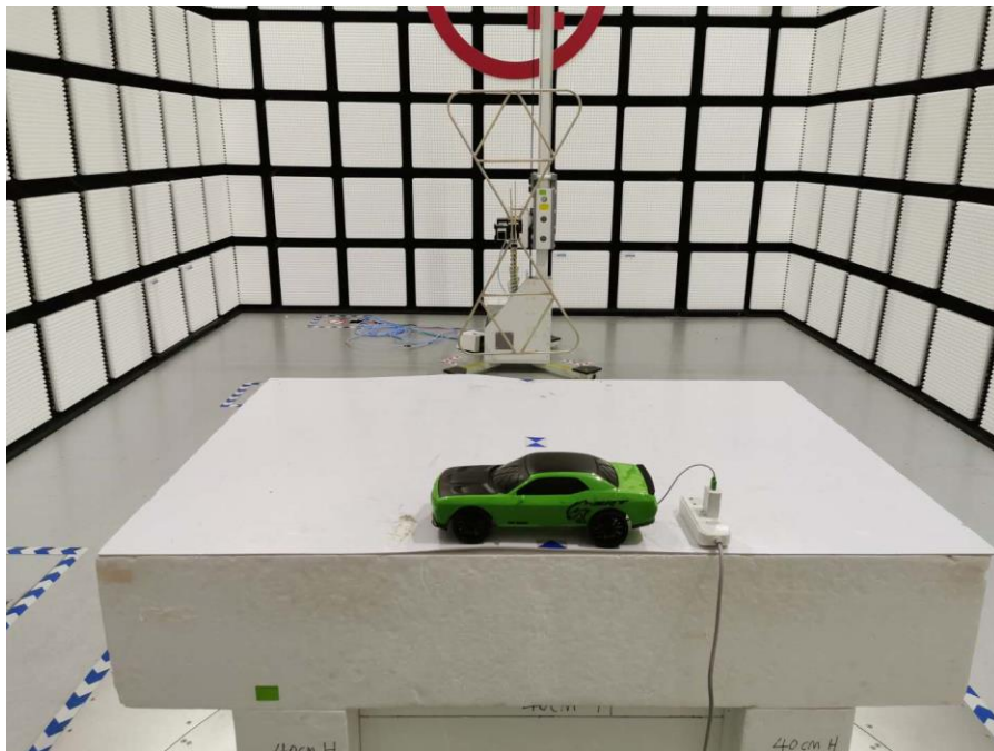
Radiated Emissions below 1GHz test setup photo
