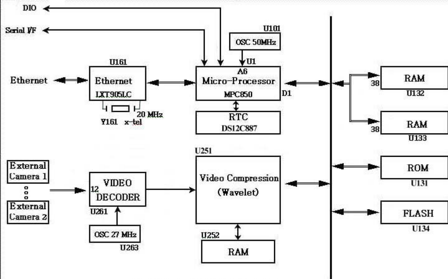
NetServer-1 Block Diagram
