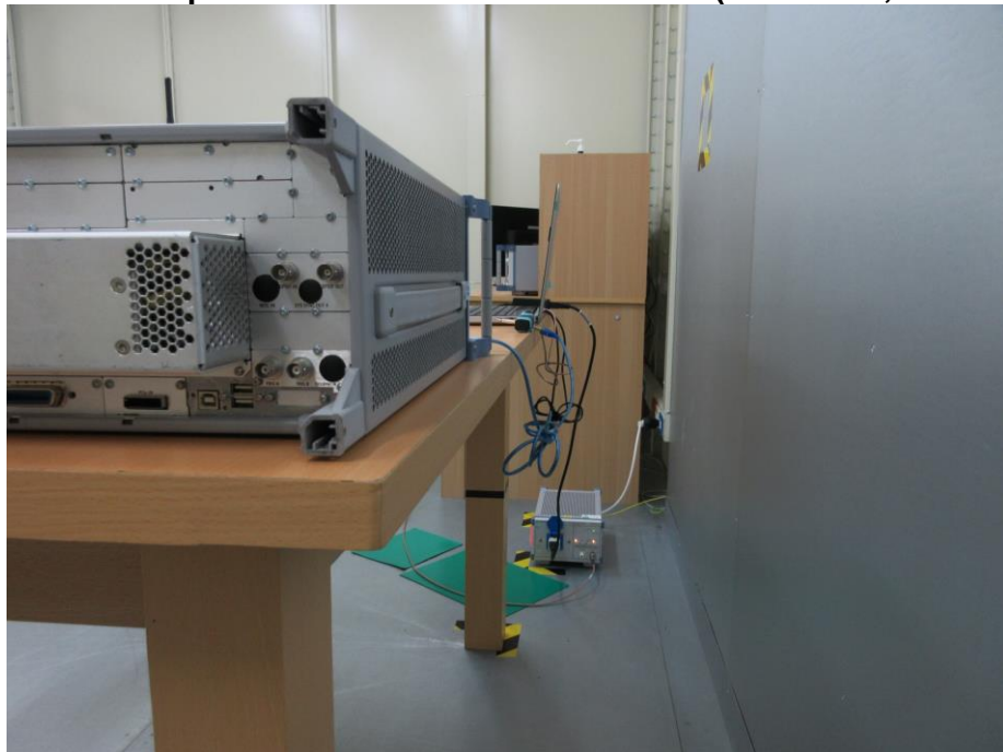
Photograph 16: Test Setup for Mains Conducted Emissions (Back View, BTM-510CD)
