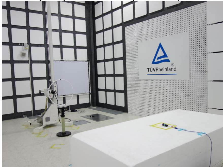
Photograph 6: Test Setup for Spurious Emissions (Back View 4, BTM-510CC)
