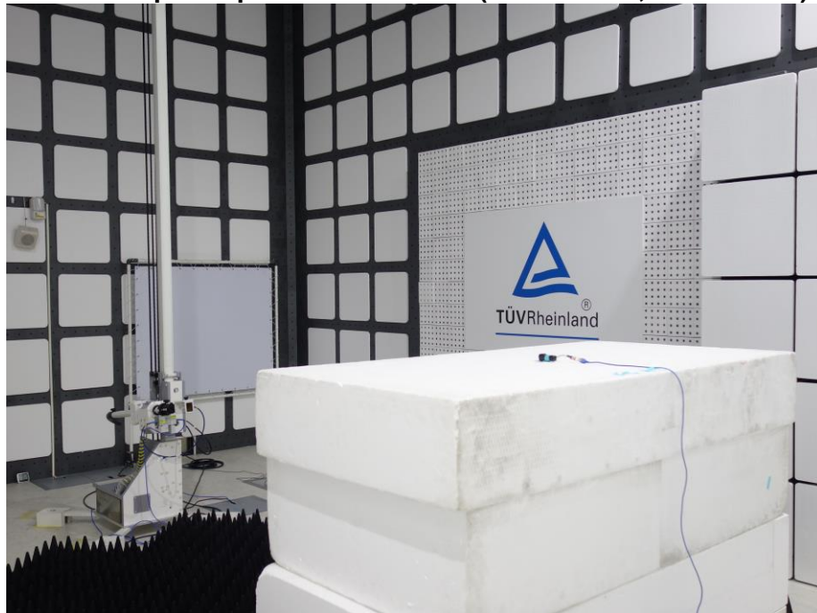
Photograph 20: Test Setup for Spurious Emissions (Back View 2, BTM-510CR)
