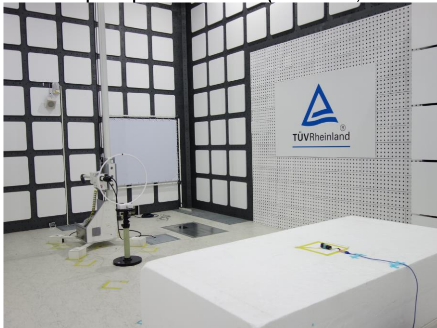
Photograph 22: Test Setup for Spurious Emissions (Back View 4, BTM-510CR)
