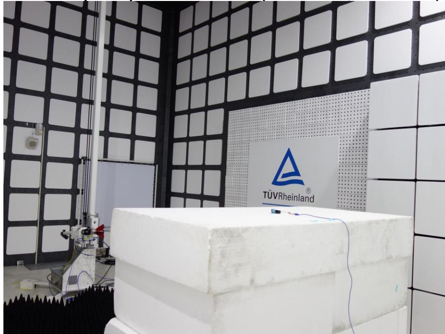
Photograph 19: Test Setup for Spurious Emissions (Back View 1, BTM-510CR)
