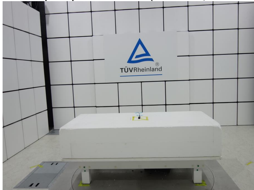
Photograph 18: Test Setup for Spurious Emissions (Front View 2, BTM-510CR)
