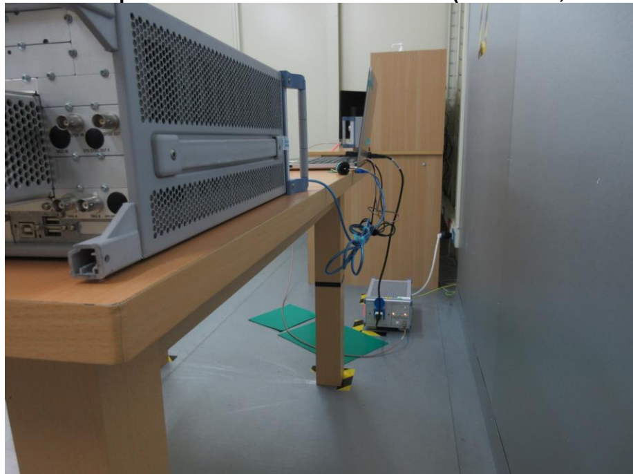
Photograph 24: Test Setup for Mains Conducted Emissions (Back View, BTM-510CR)
