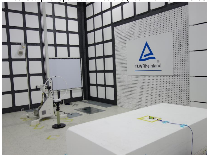
Photograph 14: Test Setup for Spurious Emissions (Back View 4, BTM-510CD)
