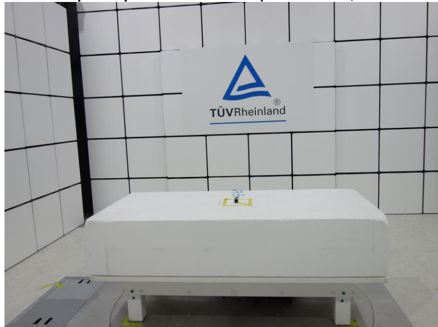
Photograph 10: Test Setup for Spurious Emissions (Front View 2, BTM-510CD)
