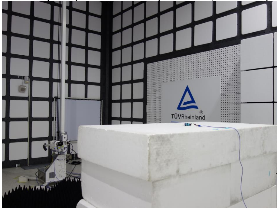
Photograph 4: Test Setup for Spurious Emissions (Back View 2, BTM-510CC)
