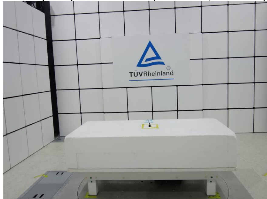
Photograph 2: Test Setup for Spurious Emissions (Front View 2, BTM-510CC)
