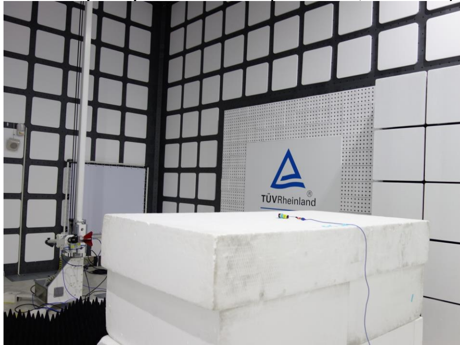
Photograph 12: Test Setup for Spurious Emissions (Back View 2, BTM-510CD)
