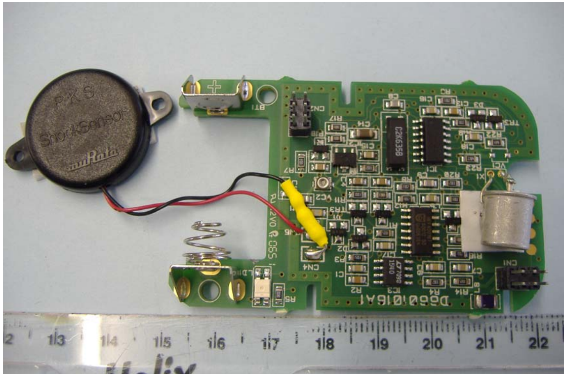
Main PCB Component Side
