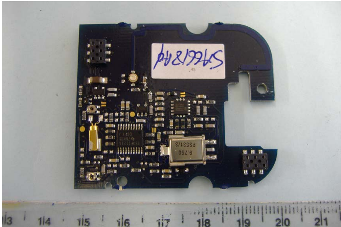
RF PCB Component Side
