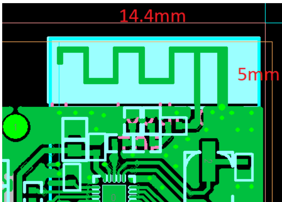
Figure 1 Physical dimension (mm)
