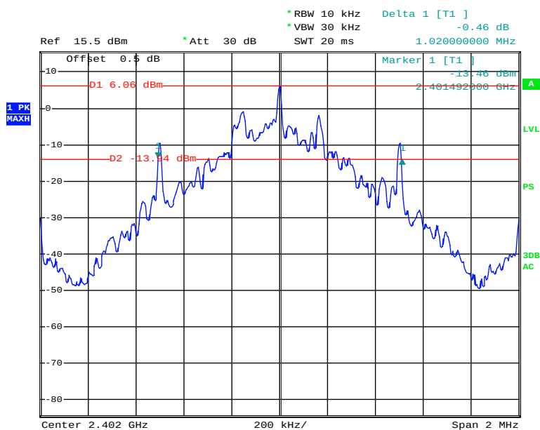
BDR (GFSK): Low Channel
