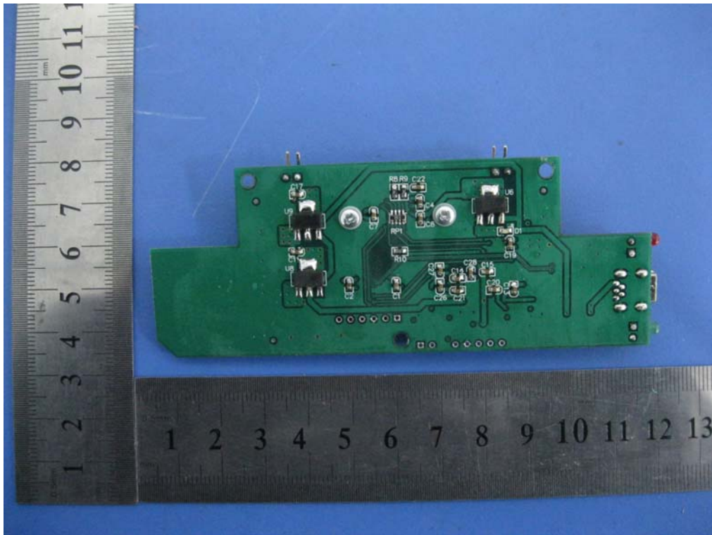
Photo #3 Rear of View- PCB Motherboard
