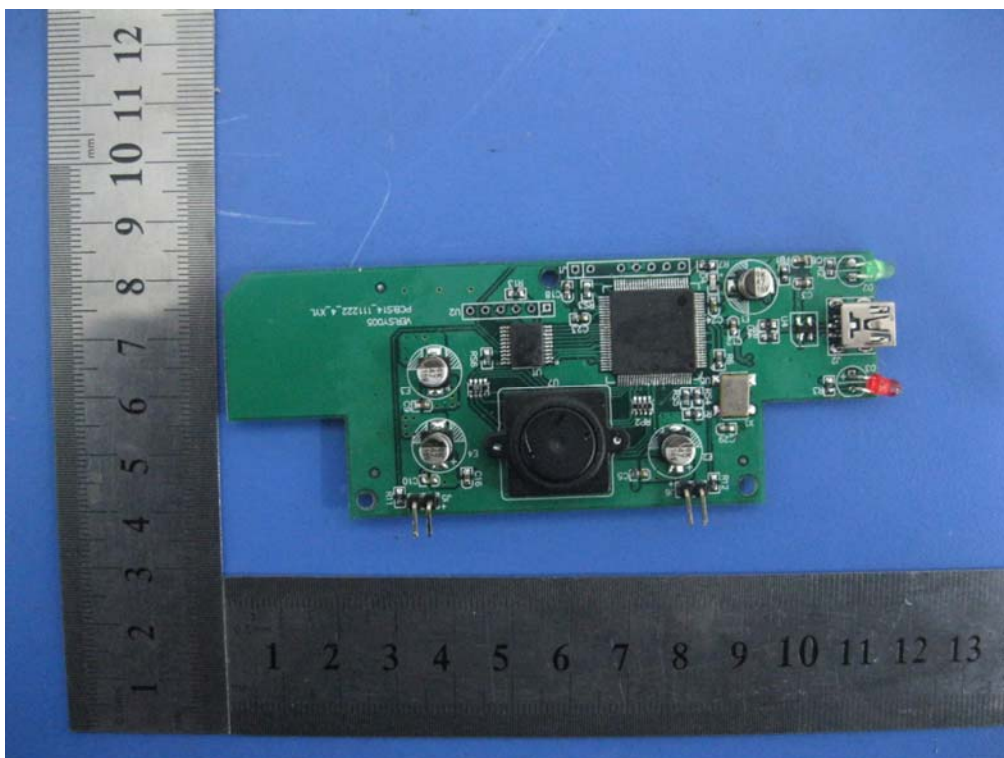
Photo #2 Front of View- PCB Motherboard
