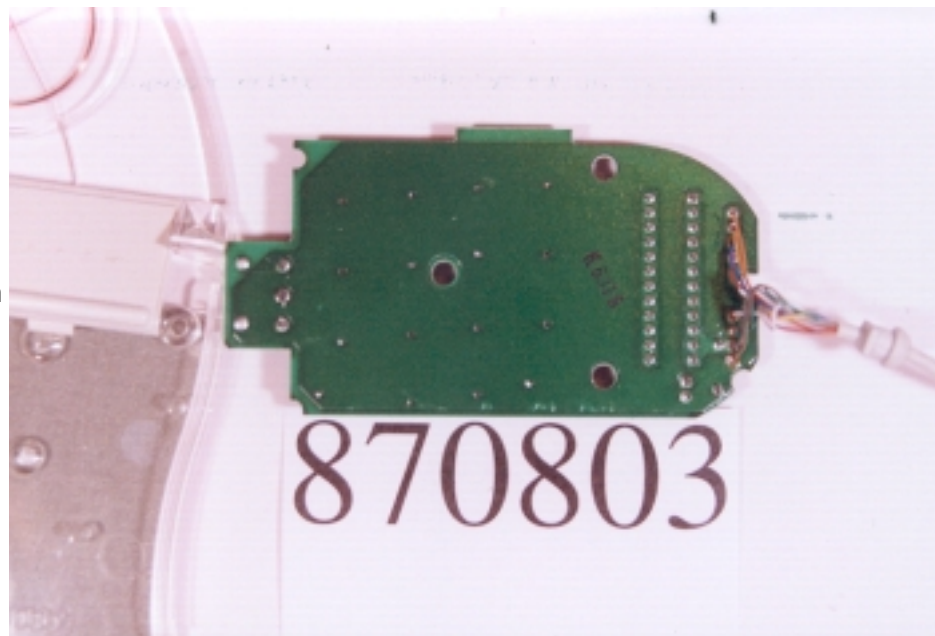
FCC ID : FSUGNWHR Rear side of main board (P04)
