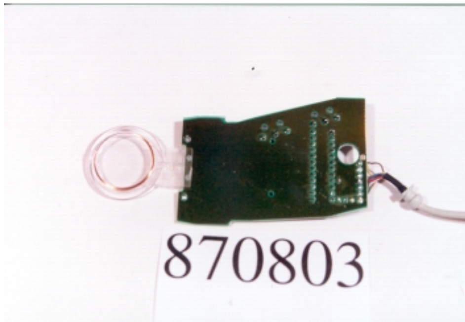
FCC ID : FSUGNWHR Rear side of main board (P07)
