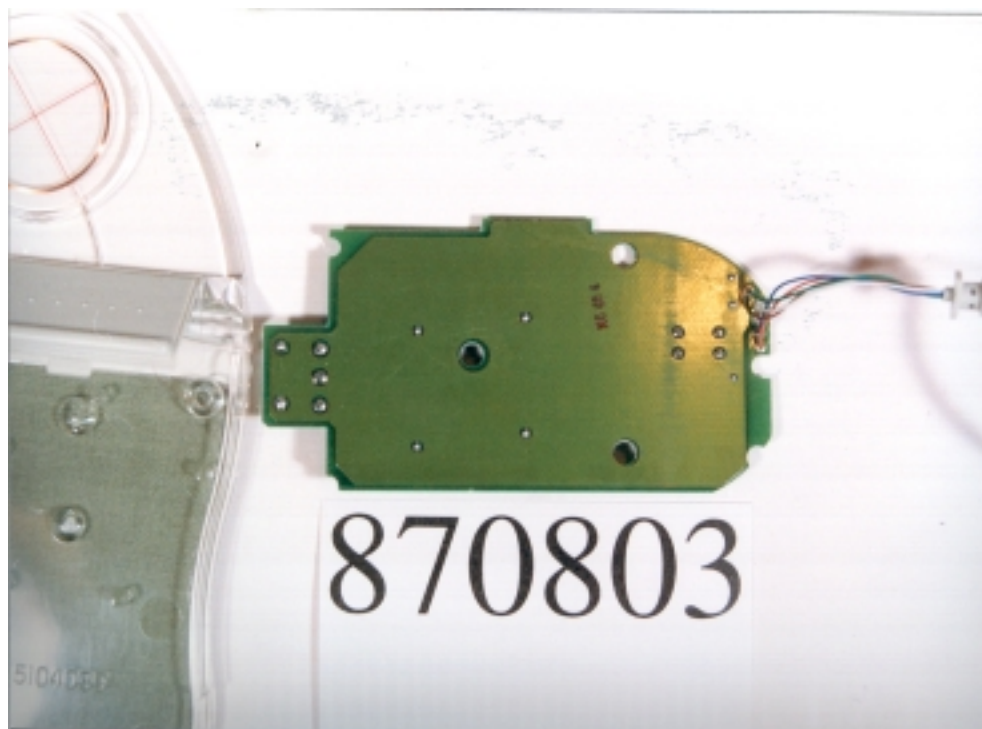
FCC ID : FSUGNWHR Rear side of main board (P05)
