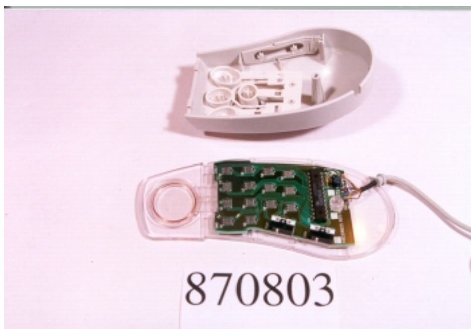
FCC ID : FSUGNWHR Mechanical Construction (P07)
