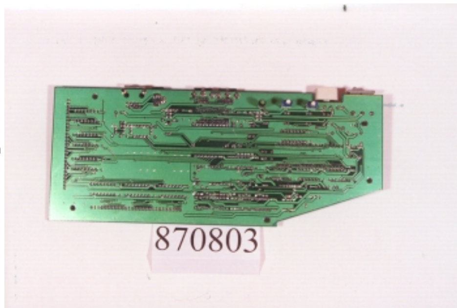
FCC ID : FSUGNWHR Rear side of main board
