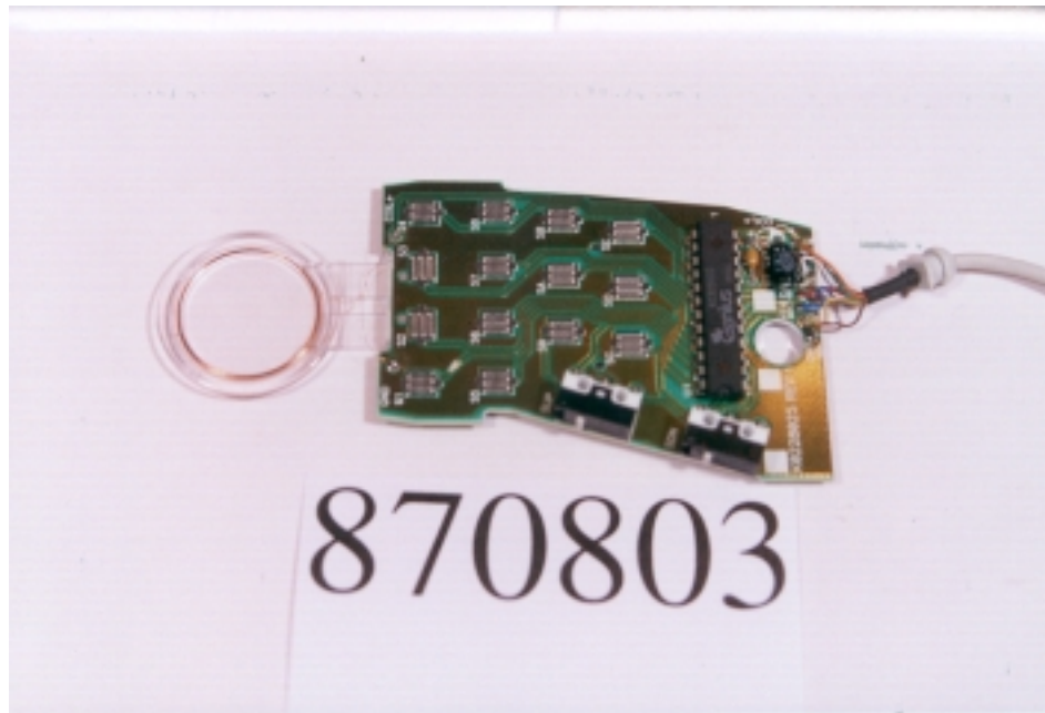
FCC ID : FSUGNWHR Front side of main board (P07)
