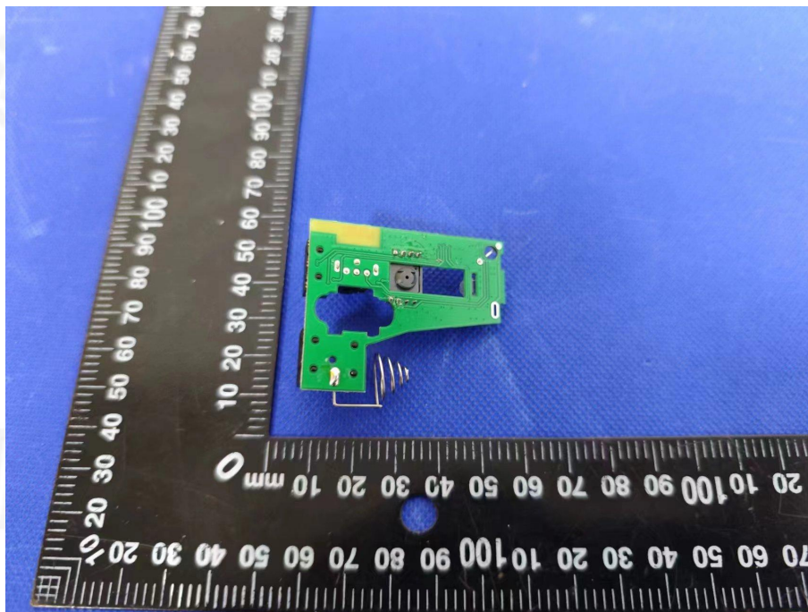
Photo 9: PCB view
