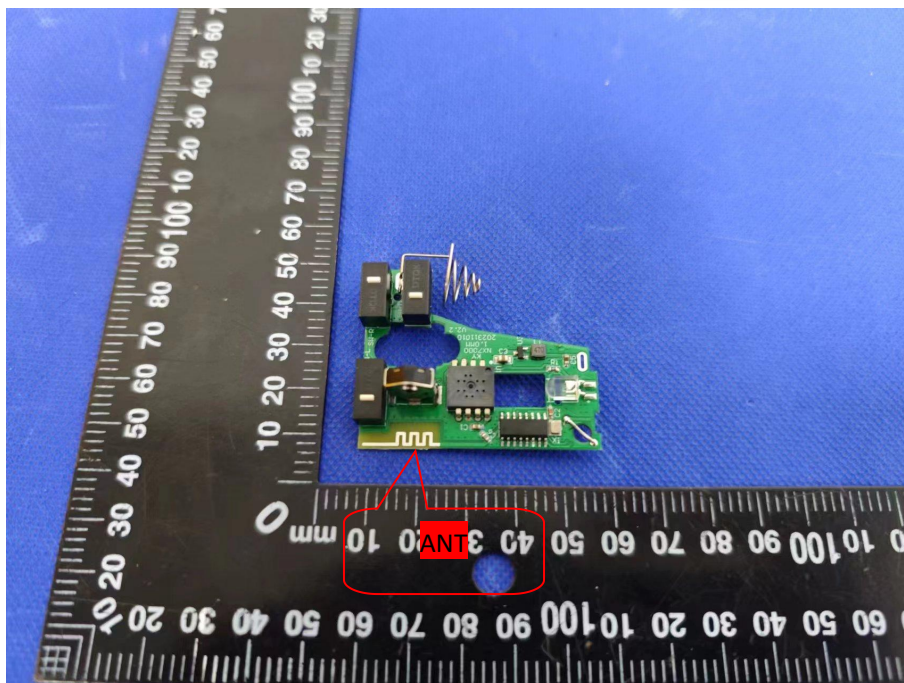
Photo 8: PCB view
