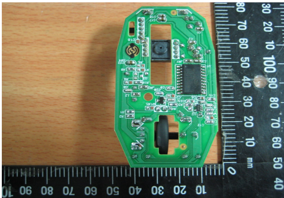
Solder Side of Main Board 1
