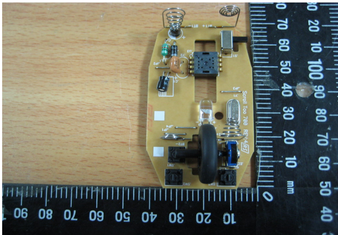
Component Side of Main Board 1
