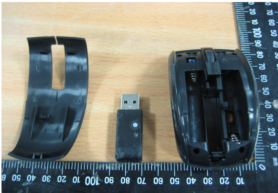
Inside View of EUT 1-1
