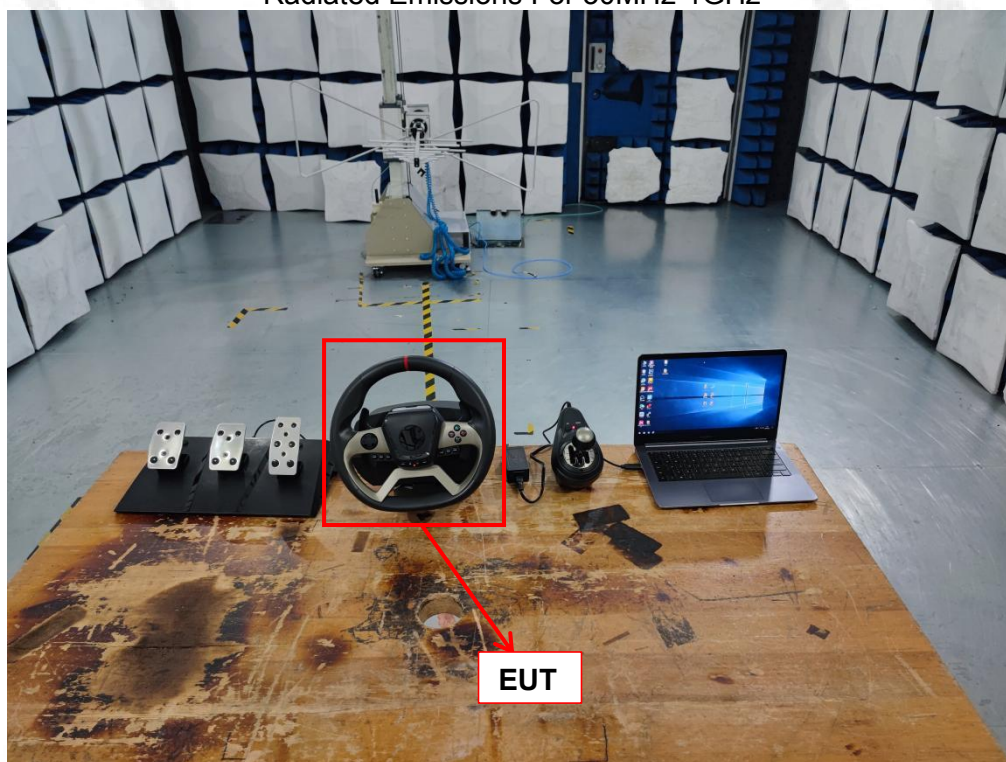
Radiated Emissions For 30MHz-1GHz
