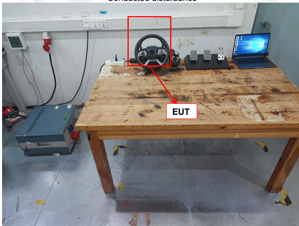
Conducted disturbance
