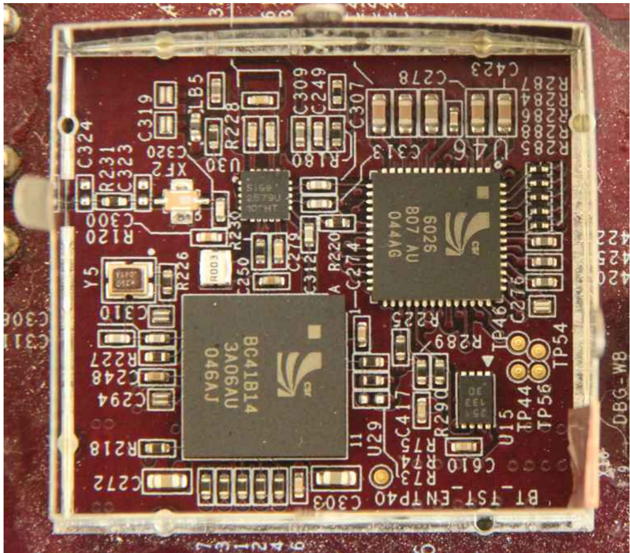
Bluetooth Section (without Screening Can) – PCB Side A (Approx x4 magnification)
