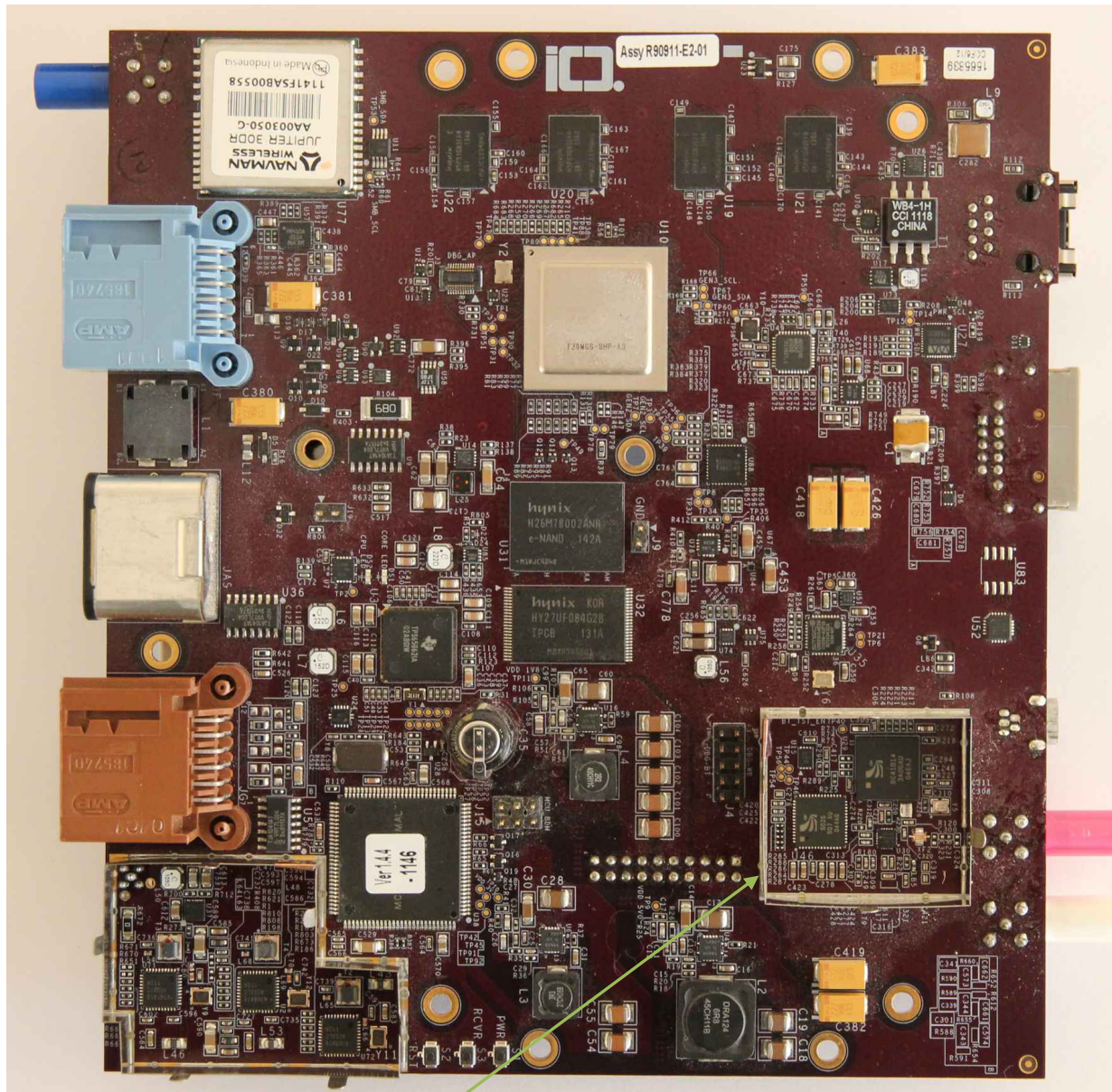
Bluetooth transceiver section
