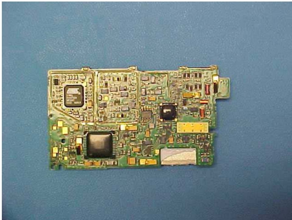
VHF RF Board without Shields - Bottom View
