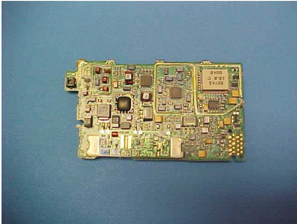
VHF RF Board without Shields - Top View
