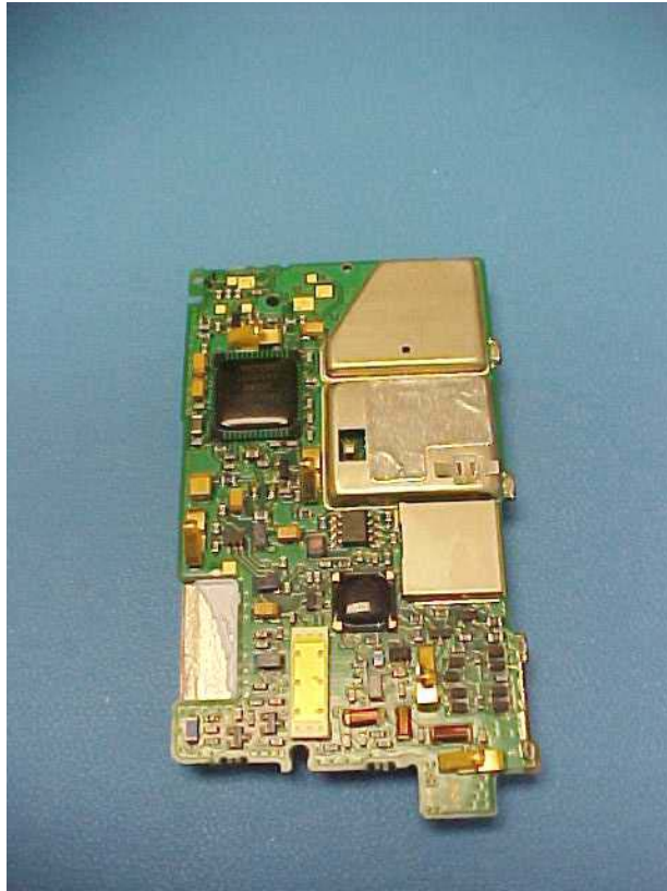
VHF RF Board with Shields - Bottom View
