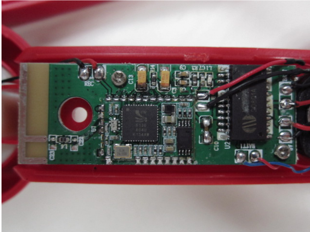
1.1.10 Rear view
