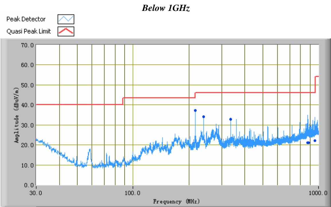
Horizontal Polarity Plot @3m
