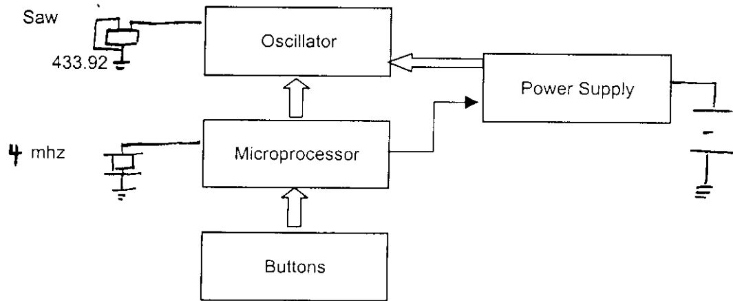
Transmitter Block Diagram
