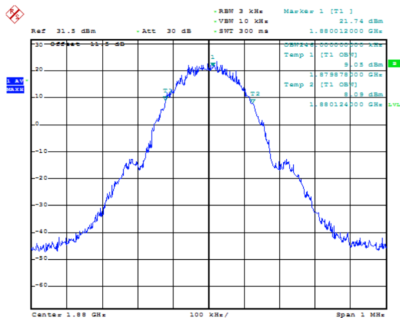
99% Occupied Bandwidth Plot on Channel 661
