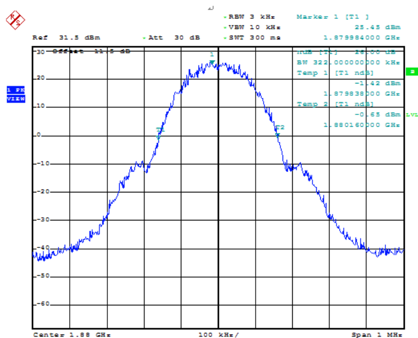
26dB Bandwidth Plot on Channel 661
