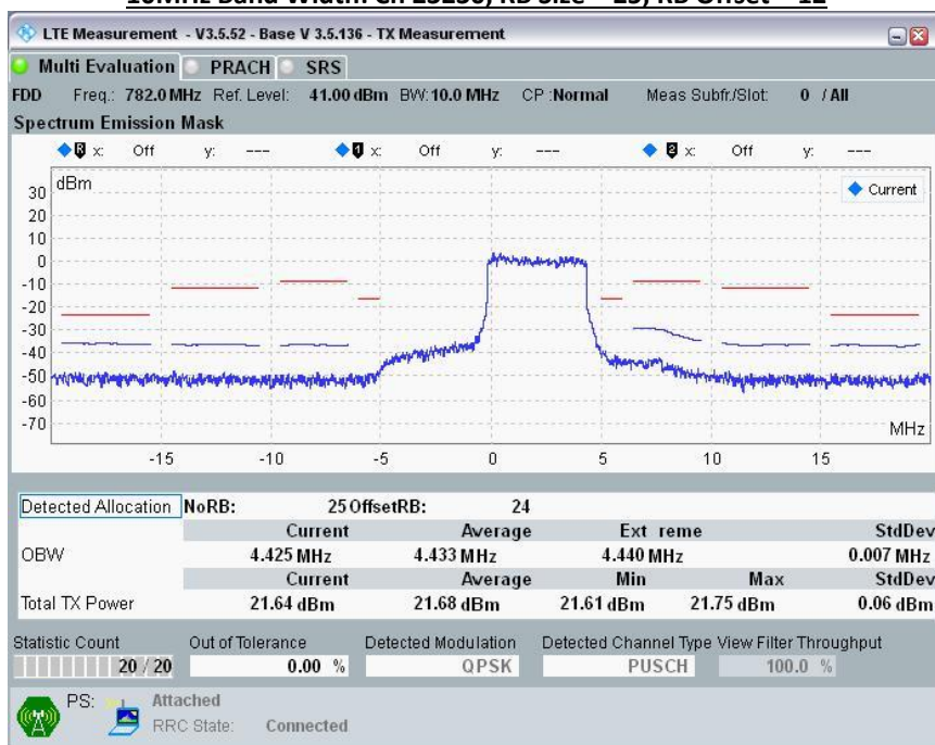
10MHz Band Width: Ch 23230, RB Size = 25; RB Offset = 24
