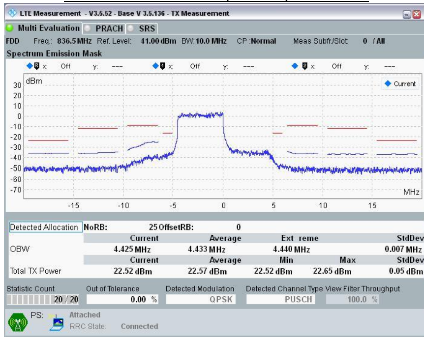
10MHz Band Width: Ch 20525, RB Size=25; RB Offset = 0
