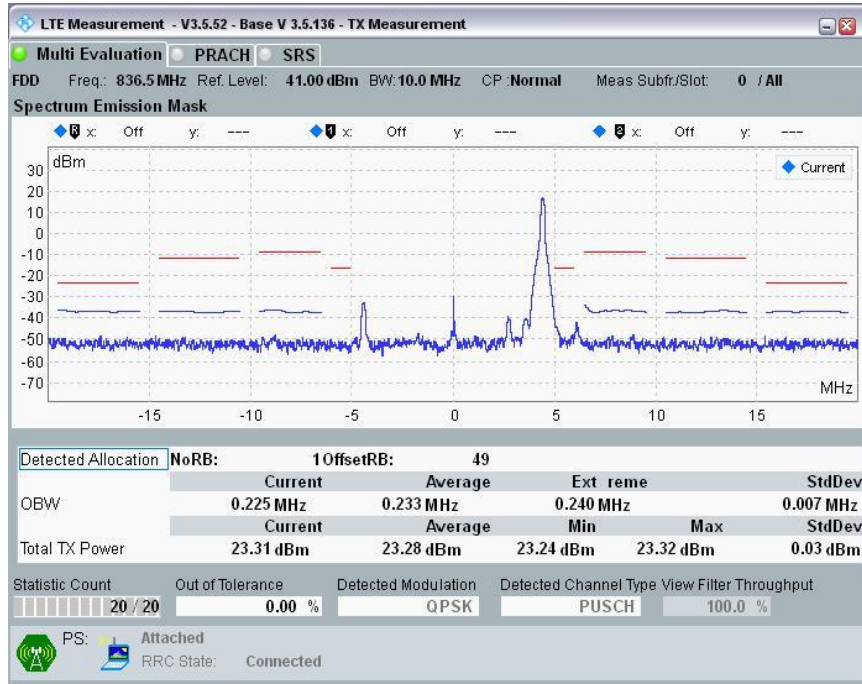
10MHz Band Width: Ch 20525, RB Size=1; RB Offset = 49
