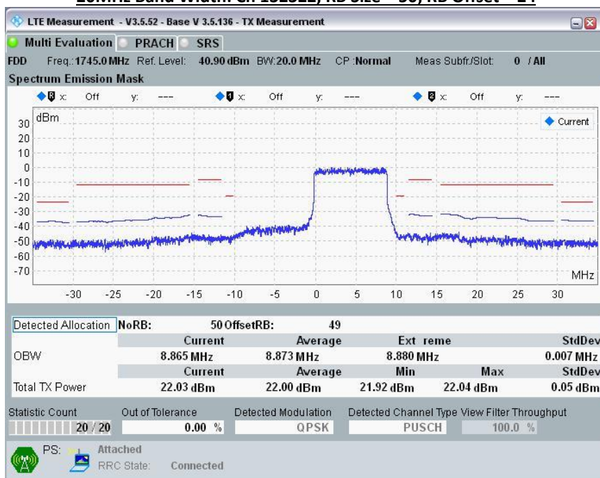
20MHz Band Width: Ch 132322, RB Size = 50; RB Offset = 49
