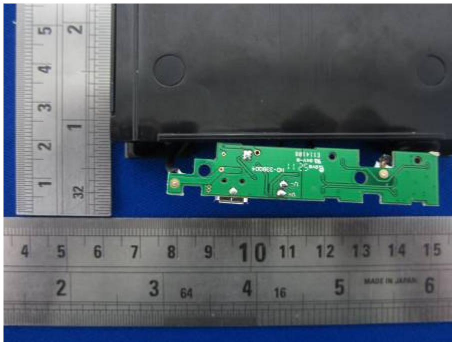
EUT –BH01u chargingbase Cover off View
