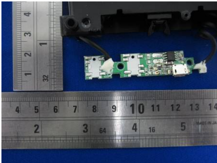
EUT –BH01i chargingbase Mainboard Top View
