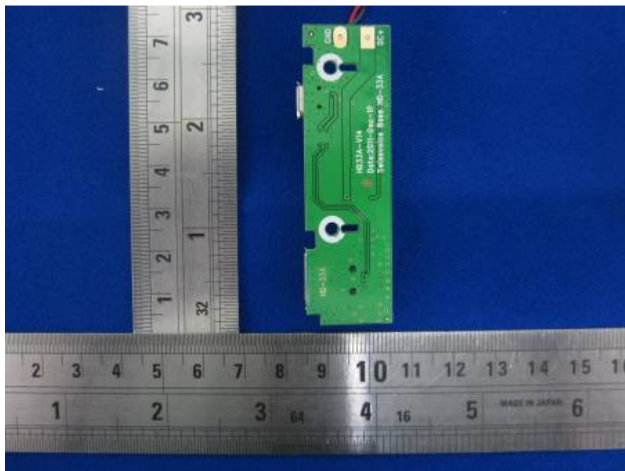
EUT –BH01u chargingbase Mainboard Bottom View
