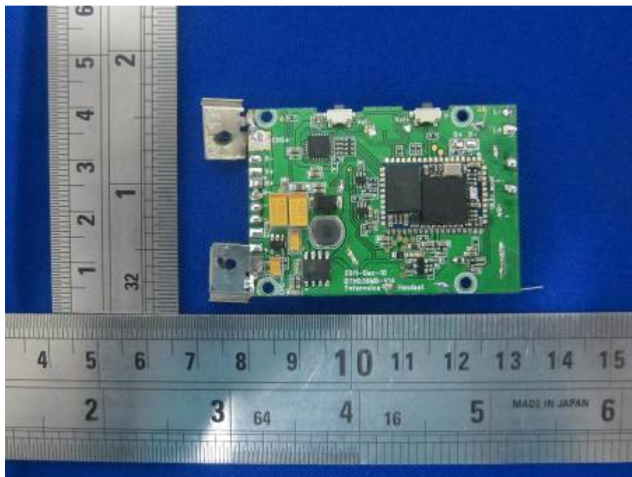
EUT –Handset PCB Top View
