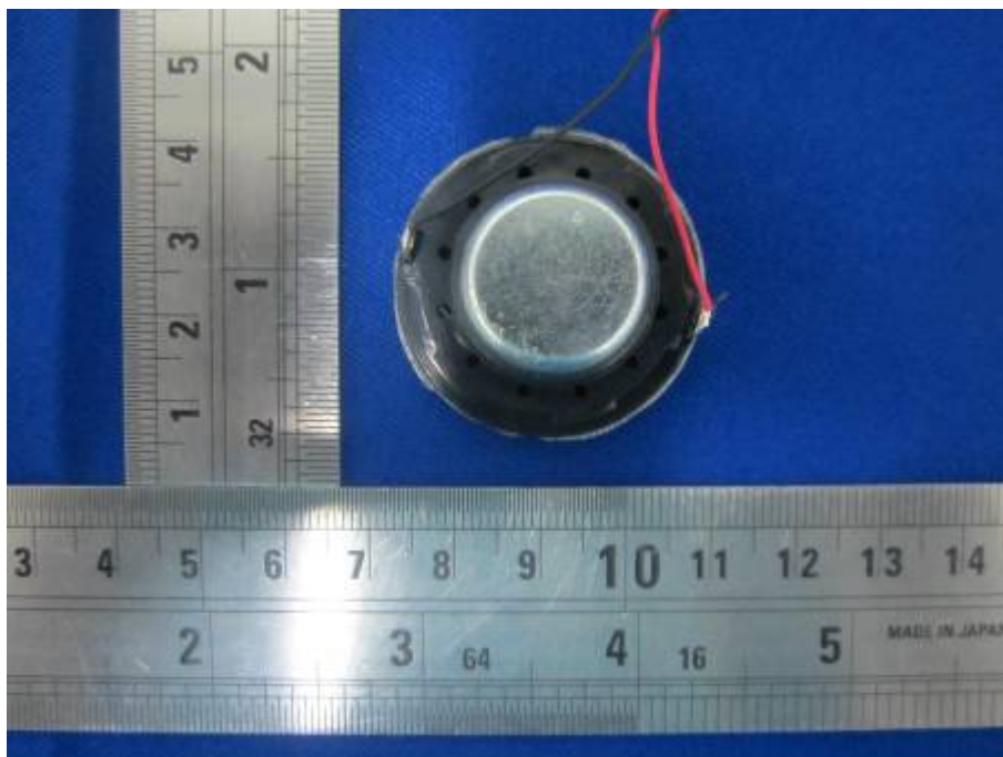
EUT –BH01i chargingbase Cover off View 1
