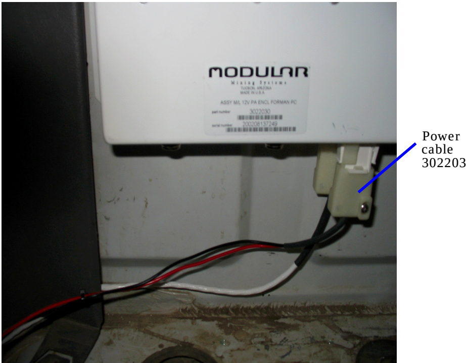
Figure 2.21 Power Cable 302203 Connected to Electrical Box
