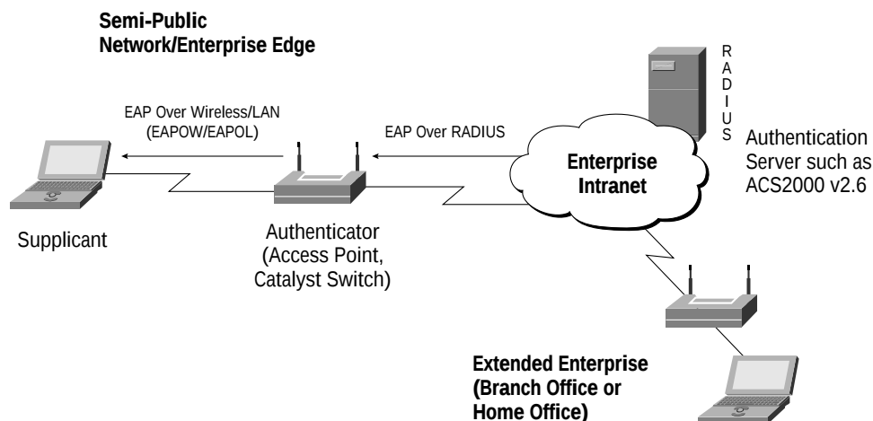
Figure 2 The 802.1x architecture implemented by Cisco is the first enterprise-ready security system for WLANs.
