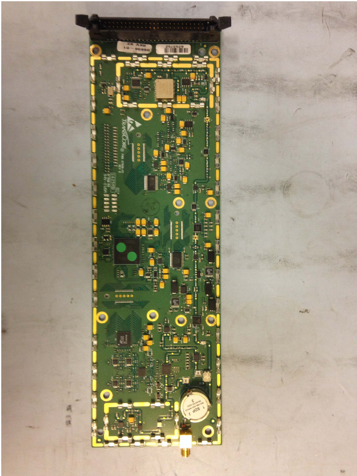
Transceiver Board Front
