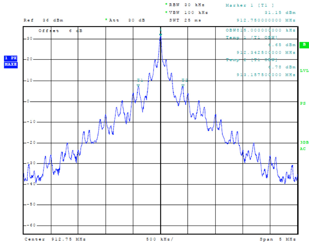
Figure 5 Occupied Bandwidth (18000-6C)
