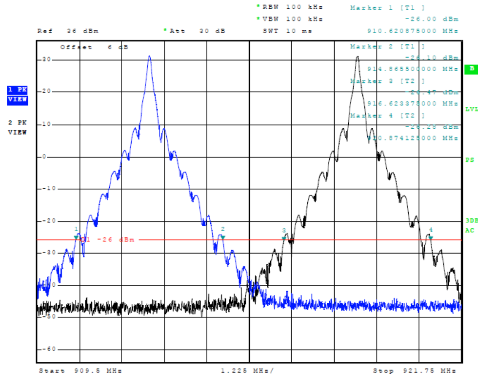
Figure 15 Emissions Mask at Antenna Terminal (18000-6C Modulation)
