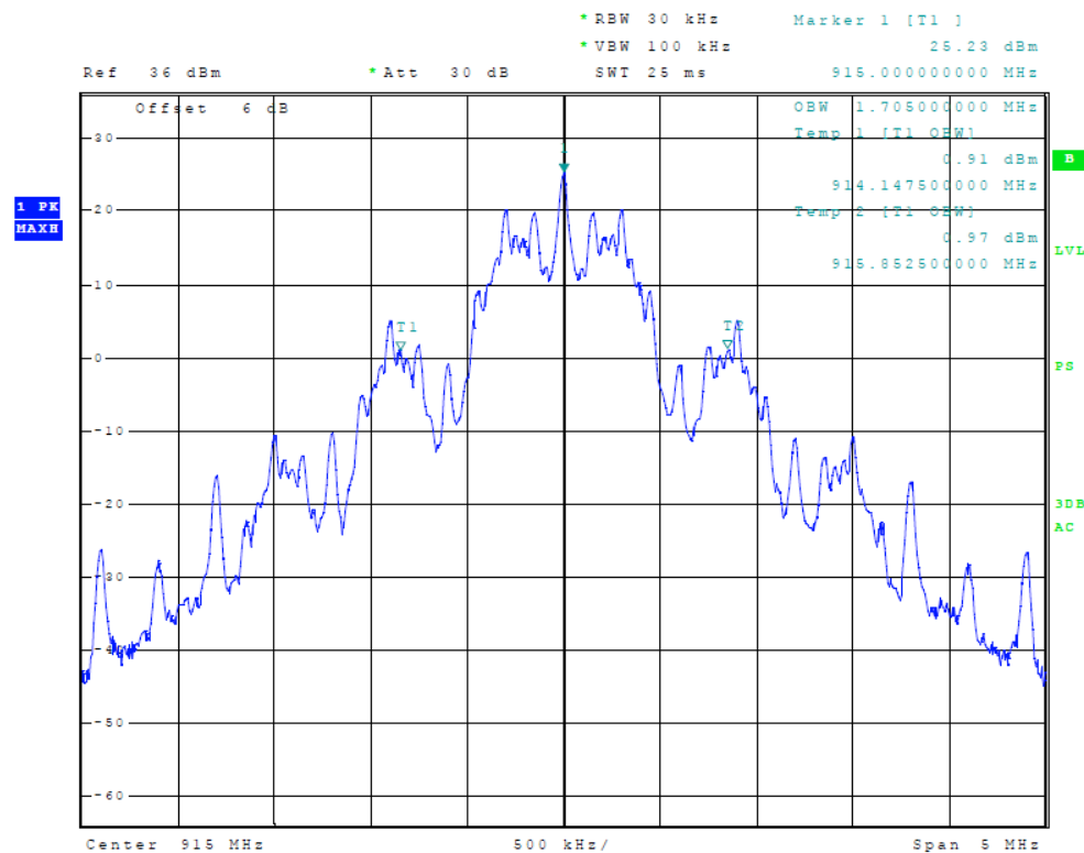
Figure 6 Occupied Bandwidth (T21)
