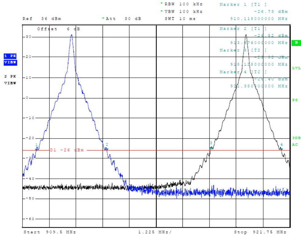
Figure 14 Emissions Mask at Antenna Terminal (SeGo Modulation)
