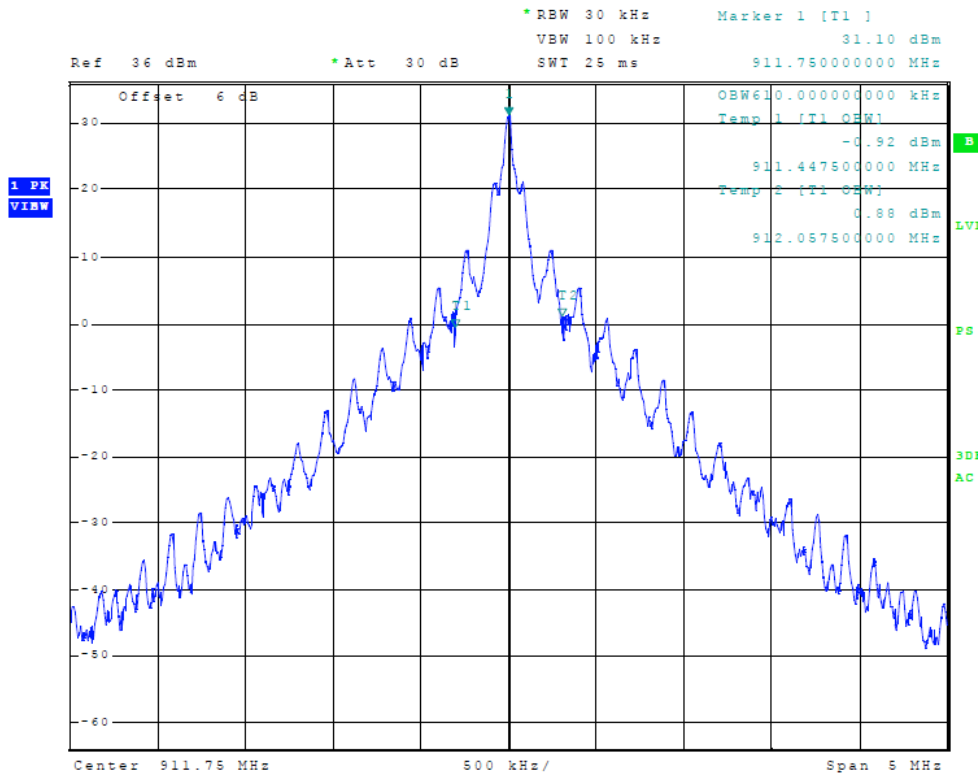
Figure 4 Occupied Bandwidth (SeGo operation)
