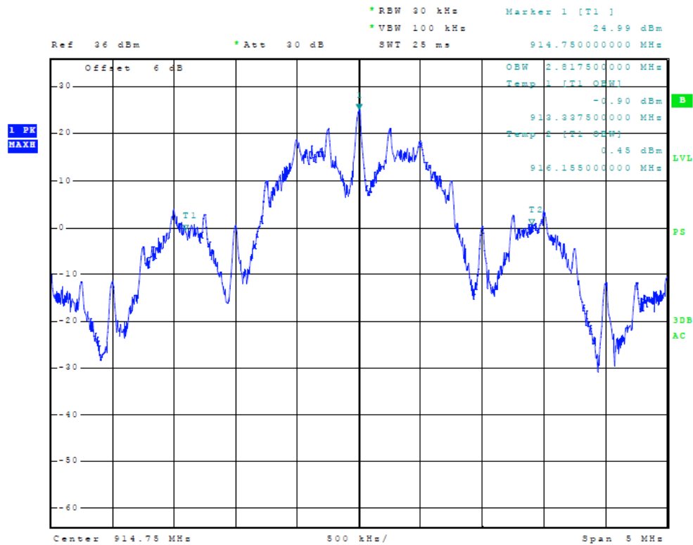
Figure 7 Occupied Bandwidth (CVISN)
