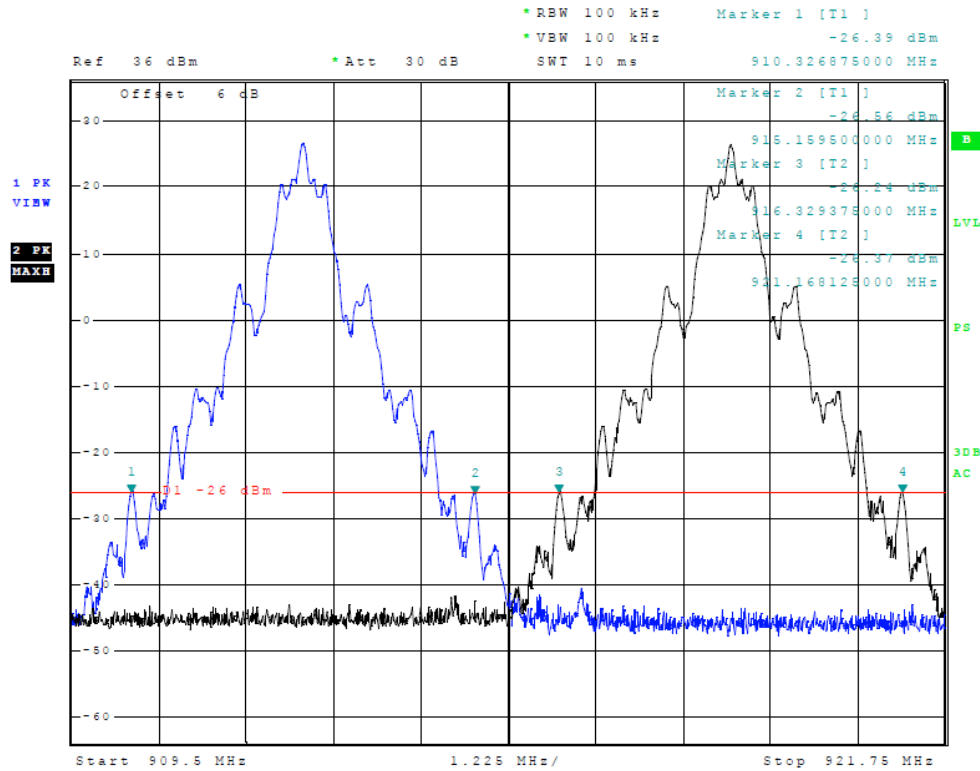
Figure 16 Emissions Mask at Antenna Terminal (T21 Modulation)
