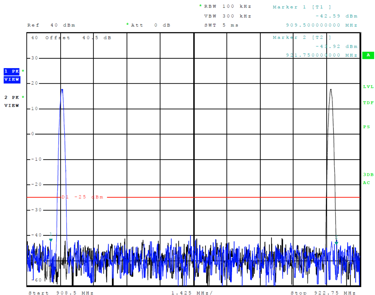
Figure 19 Emissions Mask ATA Low Power (910.00-921.75 MHz Band)
