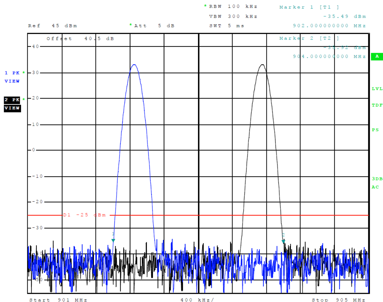
Figure 16 Emissions Mask ATA High Power (902.25-903.75 MHz Band)
