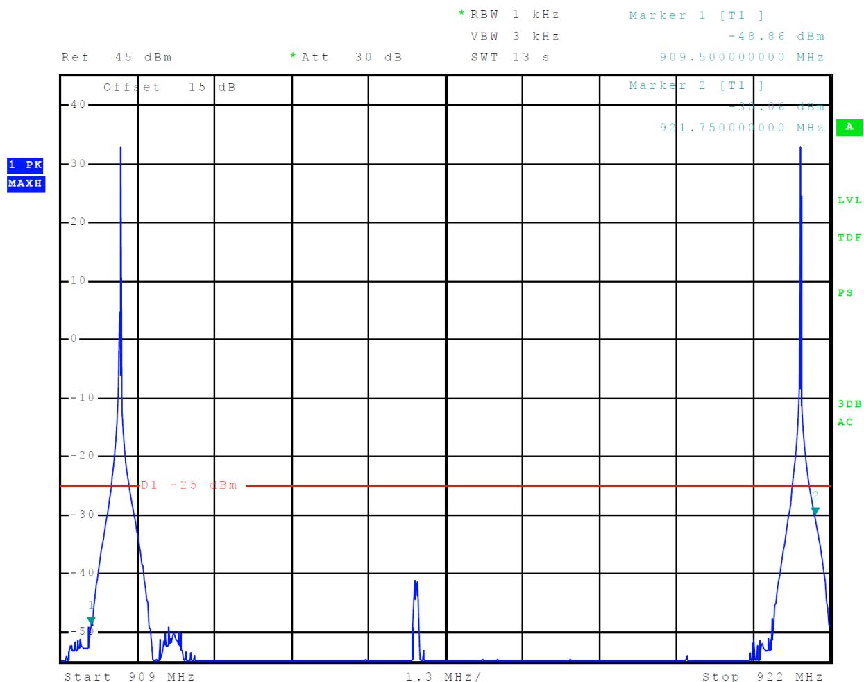
Figure 17 Emissions Mask ATA High Power (910.00-921.75 MHz Band)
