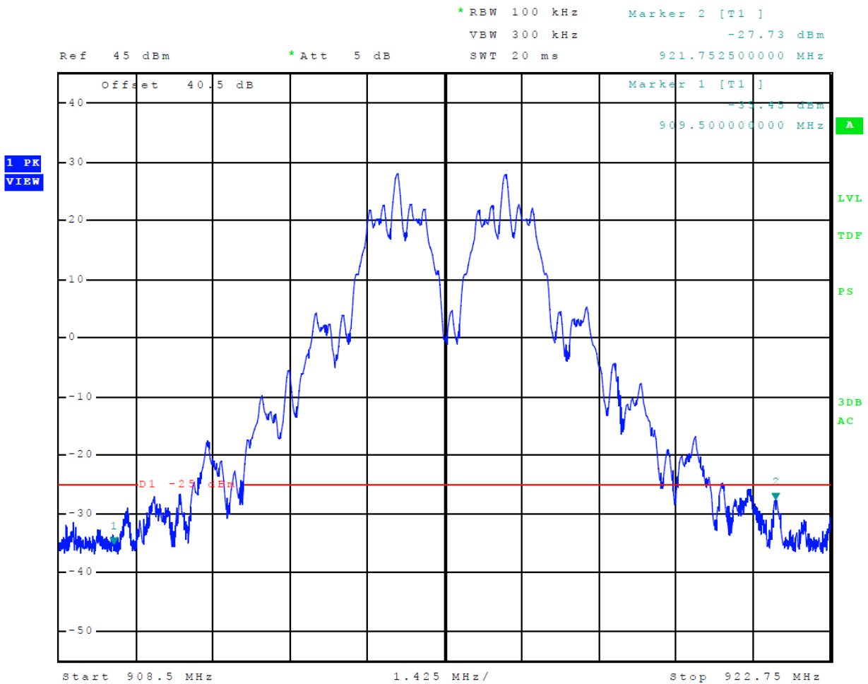
Figure 22 Emissions Mask CVS
