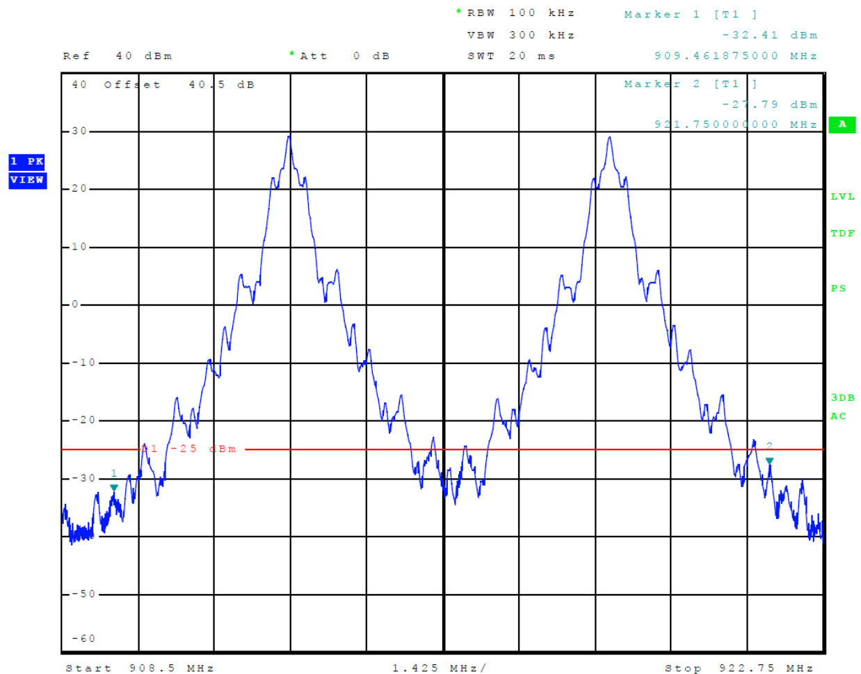
Figure 24 Emissions Mask Title 21
