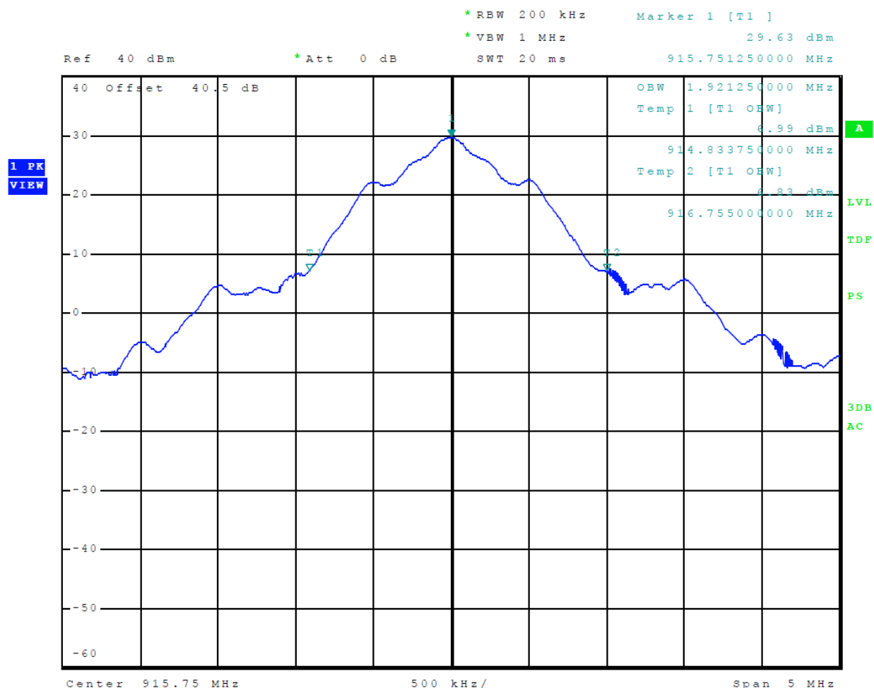
Figure 12 Occupied Bandwidth CVS
