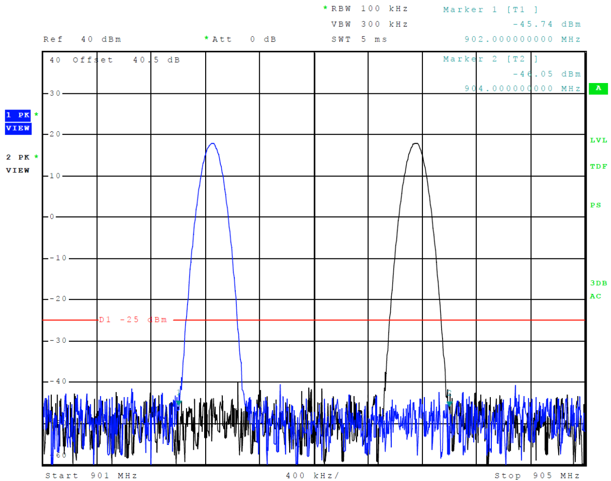
Figure 18 Emissions Mask ATA Low Power (902.25-903.75 MHz Band)
